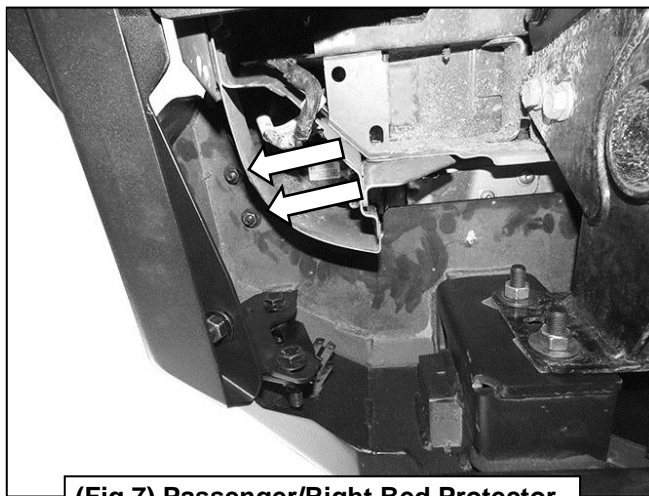
(Fig 7) Passenger/Right Bed Protector attached to the Rear Bumper
