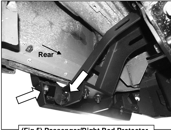
(Fig 5) Passenger/Right Bed Protector attached to the Bed Guard
