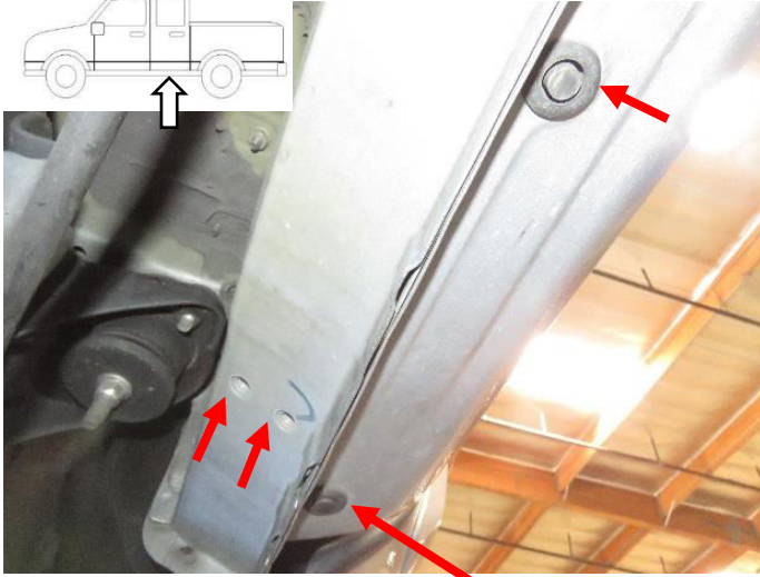
Mounting hole is very shallow
