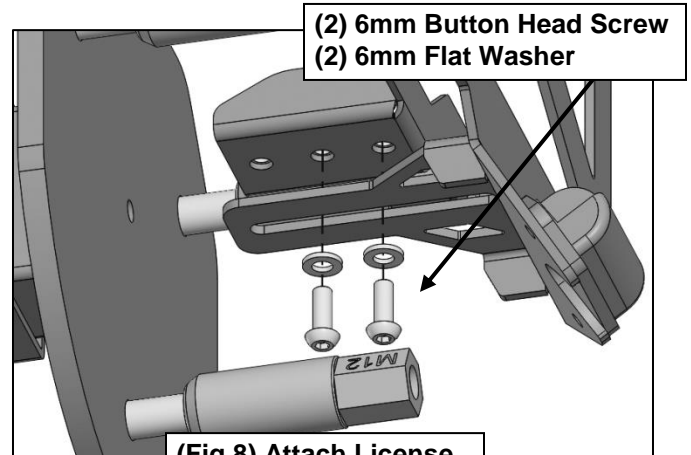
(Fig 8) Attach License Plate Mounting Bracket
