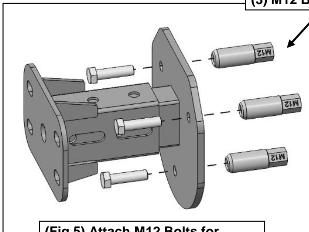
(Fig 5) Attach M12 Bolts for License Plate Bracket Installation
