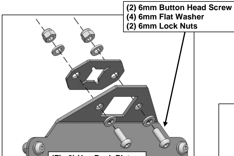
(Fig 9) Use Back Plate to attach camera to rear
