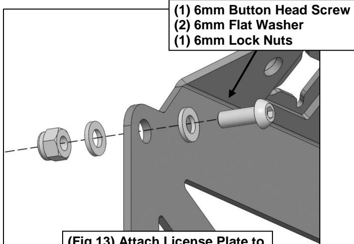
(Fig 13) Attach License Plate to License Plate Mount Bracket
