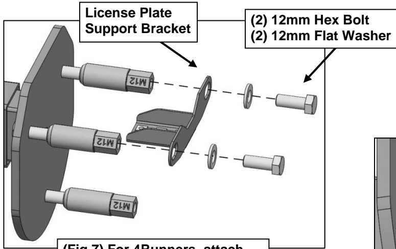
(Fig 7) For 4Runners, attach License Plate Support Bracket
