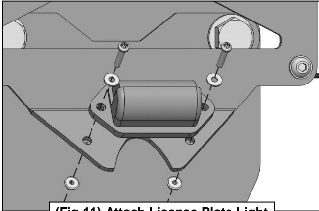
(Fig 11) Attach License Plate Light to License Plate Mount Bracket
