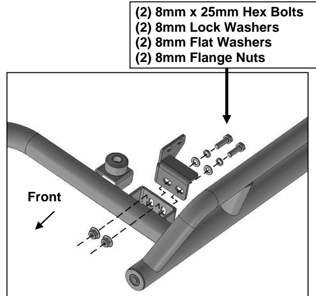
(Fig 19) Attach driver/left front Support Bracket to front end of Rocker Slider
