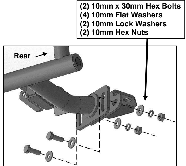
(Fig 17) Models with suspension lift "spacer," attach Adjustable Mounting Plate on end of Rocker Slider to rear Frame Bracket
