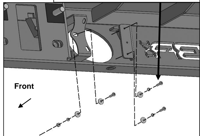
(Fig 10) Attach 3-bolt fog light assembly directly to mounting location.
