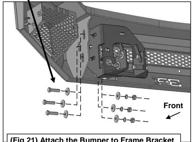
(Fig 21) Attach the Bumper to Frame Bracket
