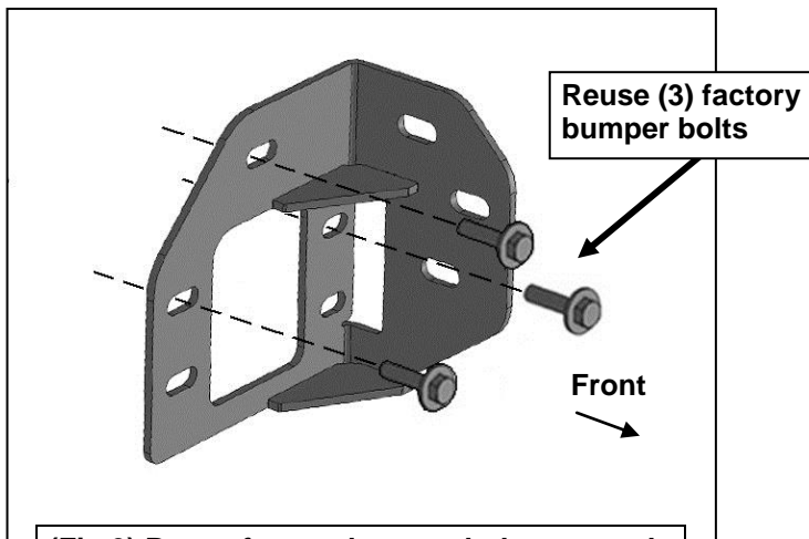
(Fig 9) Reuse factory bumper bolts to attach driver/left Frame Mounting Bracket to frame
