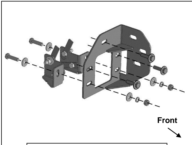
(Fig 12) Attach Support Brackets to back of Frame Mounting Bracket
