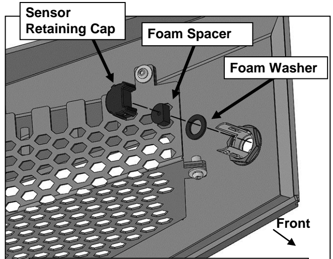
(Fig 17) Insert sensor assembly through the sensor sleeve on back of Bumper
