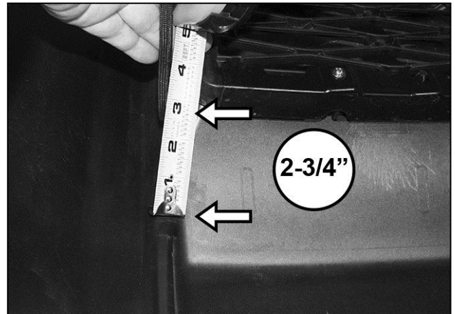
(Fig 6) Place a mark below grille on back of both sides of the bumper cover (see Figure 8)
