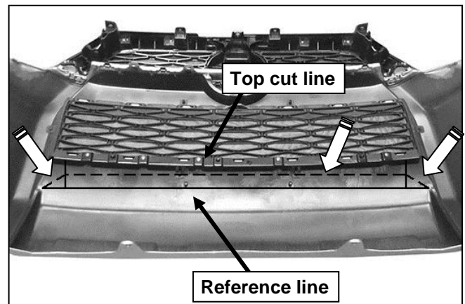
(Fig 10) Draw angled lines at the ends of the top cut line from the intersection of the vertical lines to the end of the reference line (see figures 8 & 9). The dashed line will be the horizontal top cut line (arrows). See figure 11 for vertical cut lines
