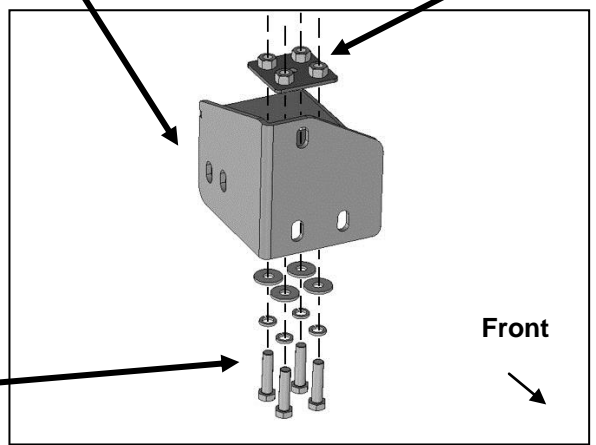
(Fig 8) Attach Mounting Brackets to frame (passenger/right Bracket illustrated)
