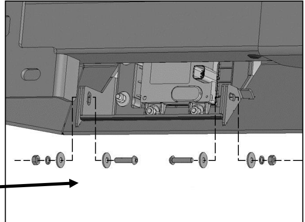
(Fig 20) Attach sensor assembly (early or late) to tabs on back of Bumper
