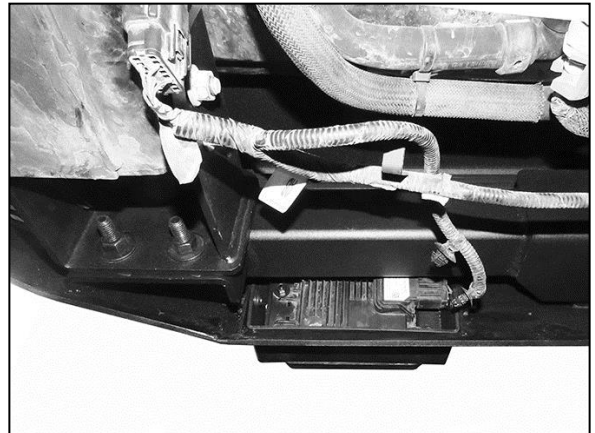
(Fig 24) Driver/left side of Bumper attached to Bumper Bracket. Sensor installation also pictured
