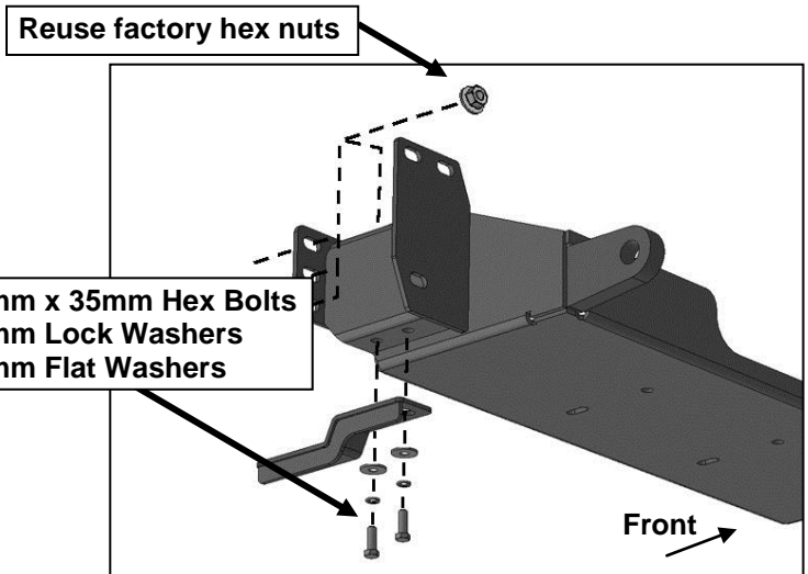
(Fig 13) Reuse factory hex nuts to attach Winch Tray Bracket Assembly to end of frame
