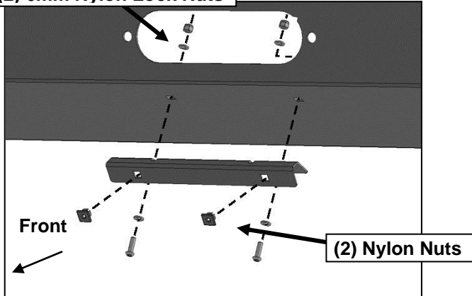
(Fig 17) Attach License Plate Bracket to Bumper
