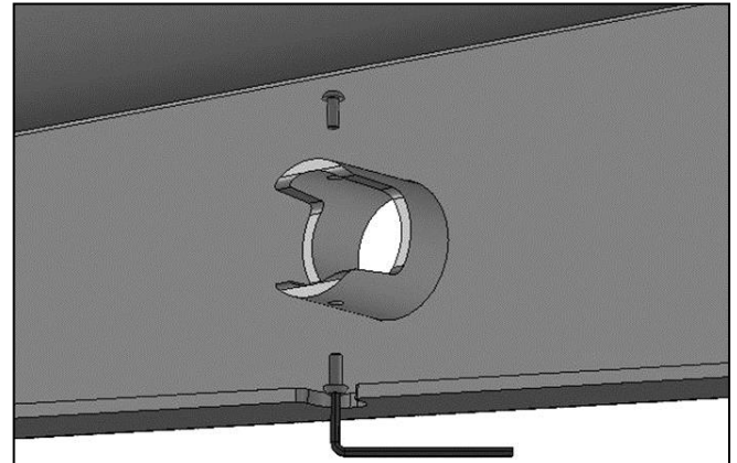
(Fig 18) Push sensor into mounting sleeve. Use 4mm Screws to lock sensor in place.
