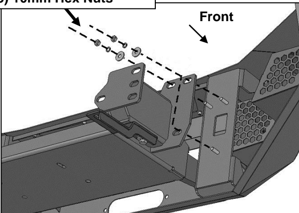
(Fig 19) Attach Bumper to Frame Brackets
