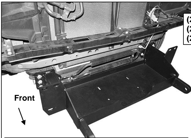
(Fig 14) Reuse factory hex nuts to attach Winch Tray Bracket Assembly to end of frame
