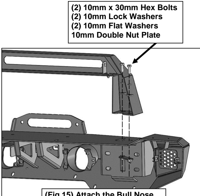
(Fig 15) Attach the Bull Nose Hoop to the top of the Bumper
