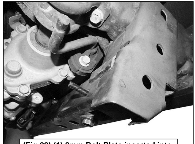
(Fig 22) (1) 8mm Bolt Plate inserted into the crossbar (Passenger/Right shown)
