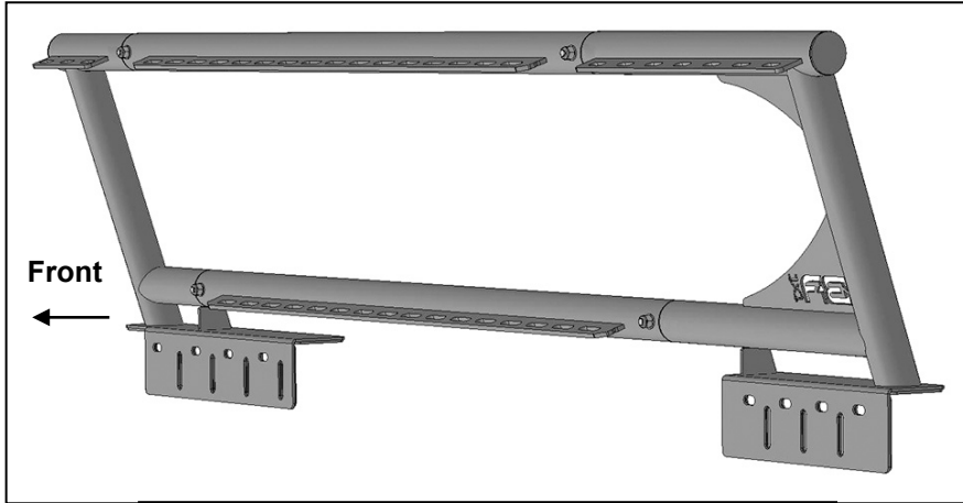
(Fig 3) Passenger/right side of Rack assembled
