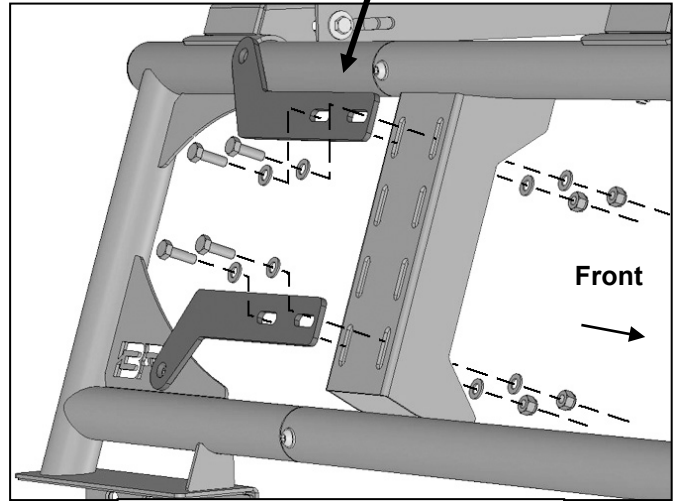
(Fig 13) Example of typical Universal "L" Bracket installation
