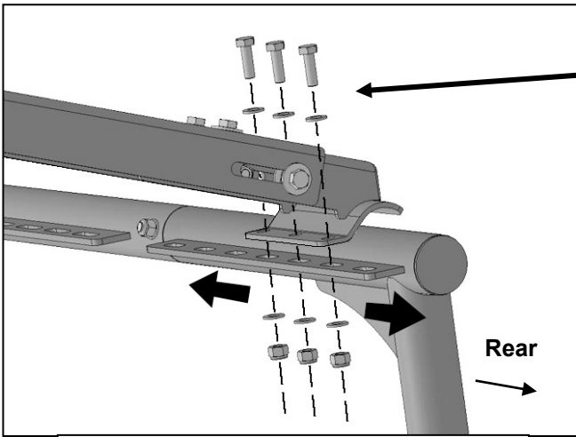
(Fig 6) Attach Cross Braces to top of front and rear Rack Ends. Do not install center Cross Brace at this time.
