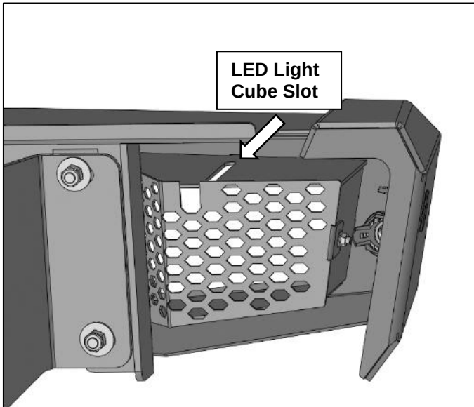
(Fig 16) Install LED cubes if available. They will be hard to install after the bumper is on vehicle.
