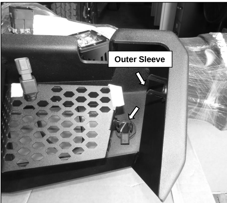
(Fig 10) If equipped, install all rear parking sensors onto Bumper. Bumpers with only four parking sensors should use inner four sleeves, with plastic cover on outer sleeves.
