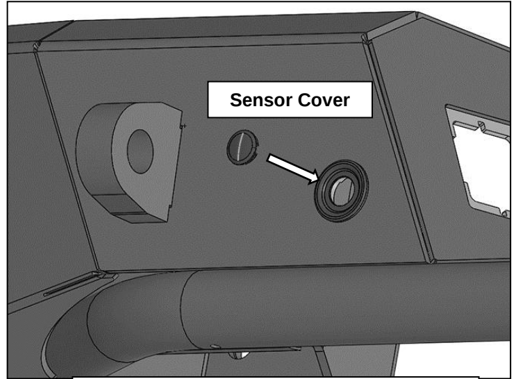
(Fig 13) If sensor sleeve does not have parking sensor installed, push sensor cover into the front of the sensor mounting sleeve
