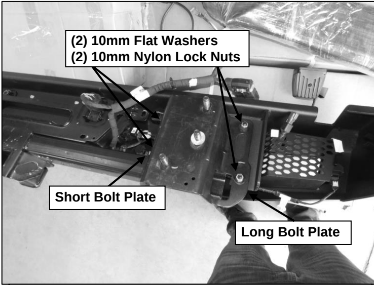
(Fig 22) After: Place hitch receiver with bracket onto bumper, then insert Short 10mm Double Bolt Plate on inner side to secure bracket while allowing Long 10mm Double Bolt plate to slot through hitch receiver slots. Use hardware to secure hitch receiver to Long 10mm Double Bolt Plate
