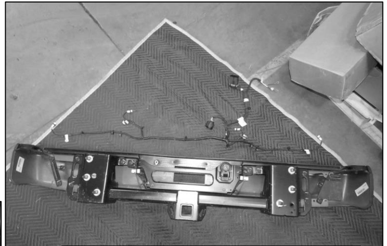
(Fig 6) Disassemble the bumper to remove sensors, (if equipped), license plate lights, trailer plug, and wiring harness.
