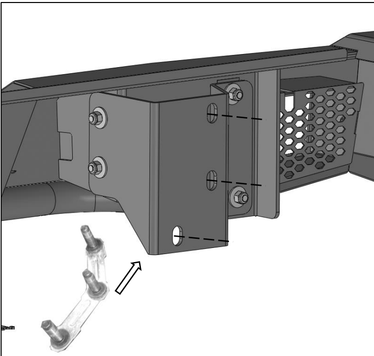
(Fig 24) Install Factory Triple Bolt Plate behind bracket. Use factory retaining clips to keep factory bolt plate in place.
