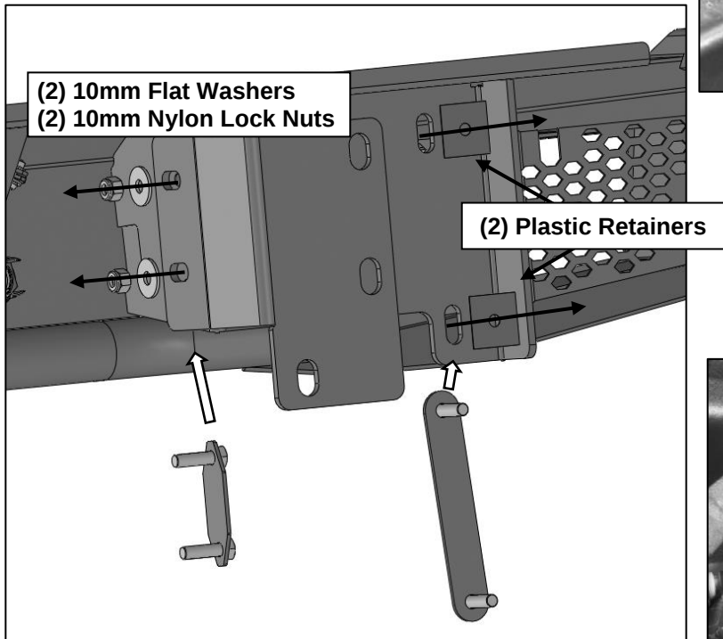
(Fig 20) Insert Long 10mm Double Bolt Plate into the back of Bumper. Use 10mm Plastic Retainers to hold Bolt Plate in position, and secure Short Double Bolt Plate with indicated hardware to secure bracket installed on hitch receiver. See Fig for Before and After.
