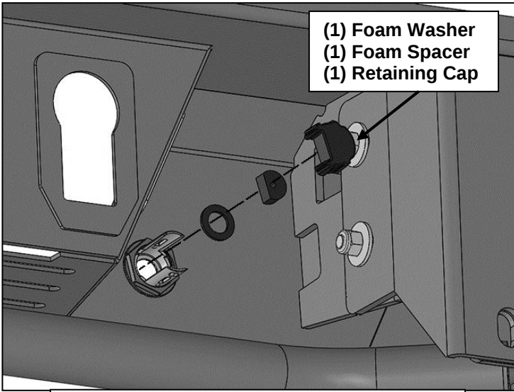
(Fig 12) Secure parking sensor using indicated hardware from back of bumper
