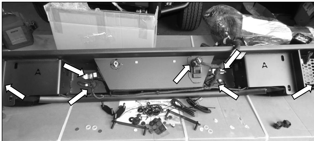
(Fig 17) Plug main wire harness to all parking sensors, both license plate lights, and trailer plug
