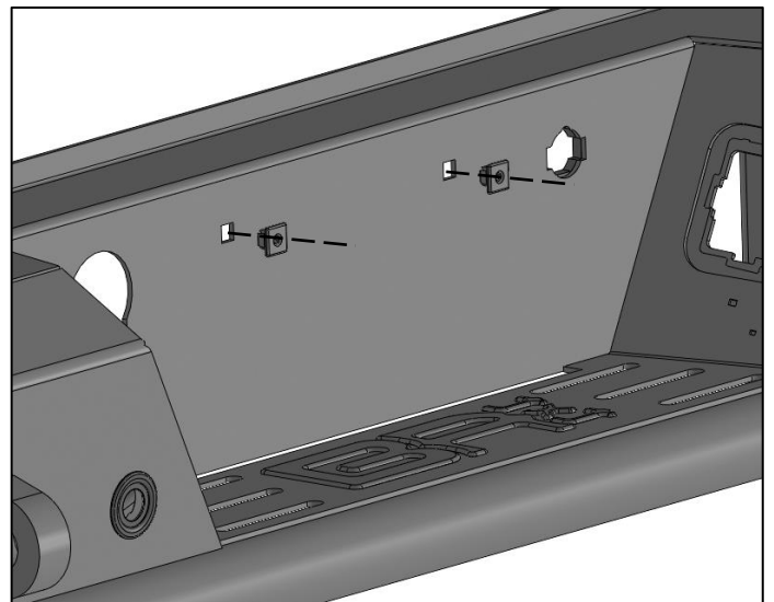
(Fig 27) Insert square plugs for license plate and reinstall license plate.
