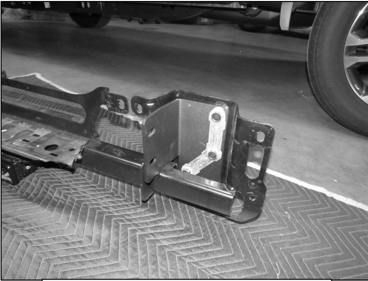
(Fig 18) IMPORTANT: FOR VEHICLES WITH TOW HOOK PACKAGE ONLY , install brackets onto hitch assembly using factory triple bolt plate
