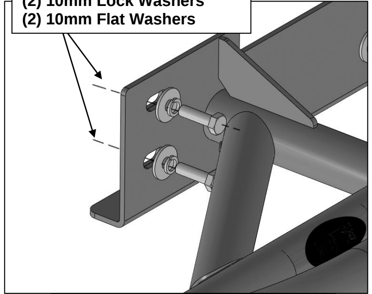
(Fig 8) Mount rear bracket using indicated hardware
