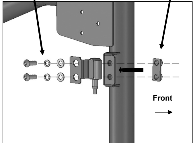
(Fig 5) Attach (2) Passenger/right Hinges to Door
