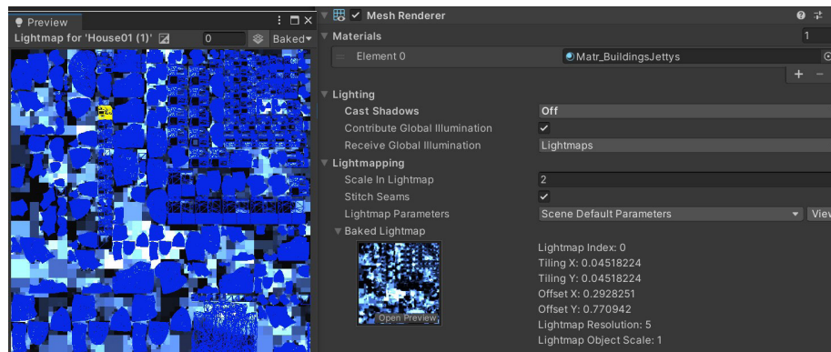
Adjust the Lightmapping Settings ( Windows > Rendering > Lighting Settings ) and Lightmap size to limit memory usage.
