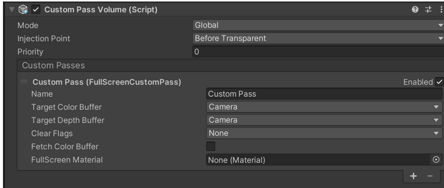
A CustomPassVolume in HDRP.
