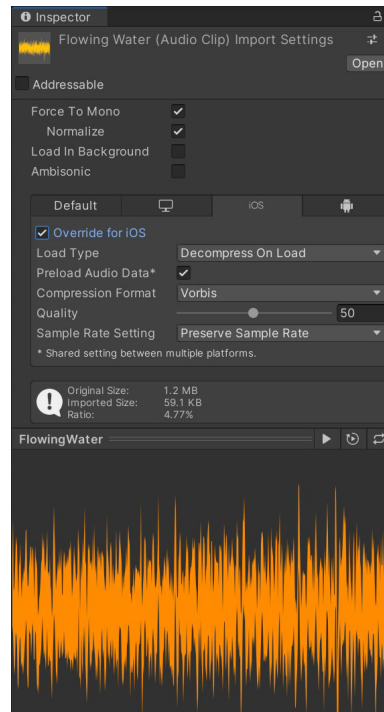
AudioClip Import Settings
