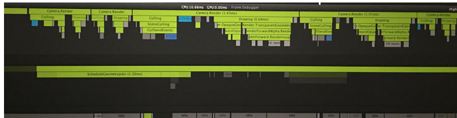
The Unity CPU Profiler shows the main thread in the timeline view and indicates that there are multiple Cameras. Unity performs culling for each Camera.
