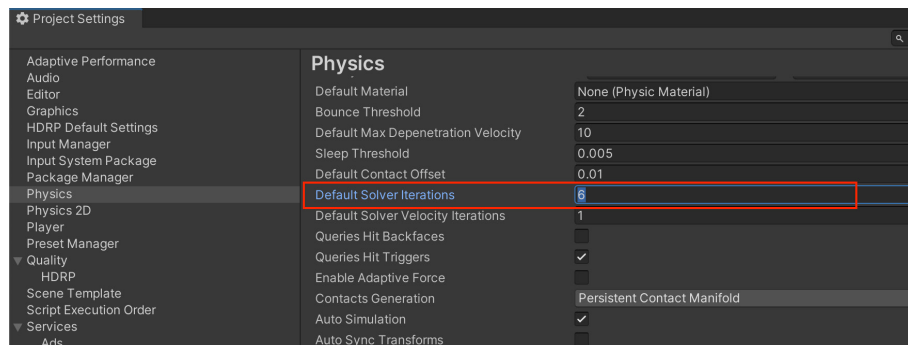
Override the defaultSolverIterations per Rigidbody
