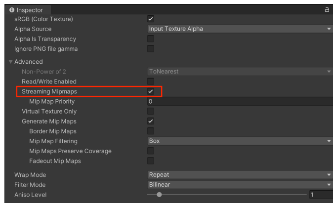
Streaming Mipmaps is enabled.
