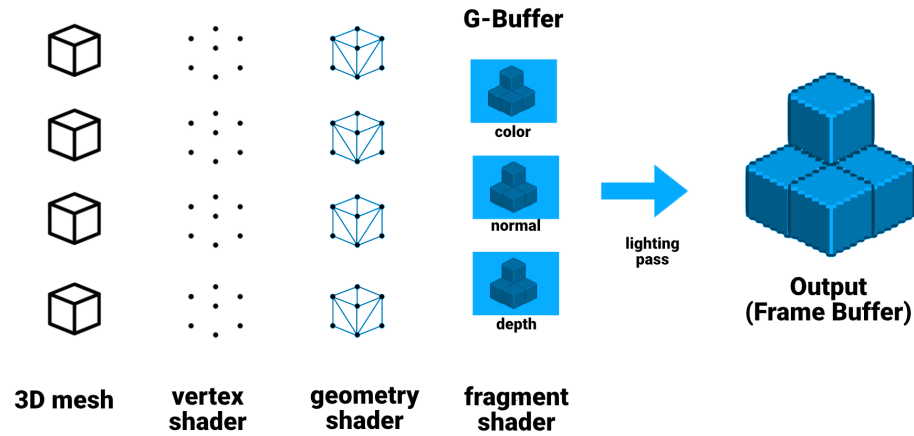
Deferred shading path
