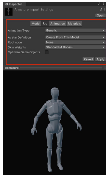
Generic rigs use less CPU time than humanoid rigs.
