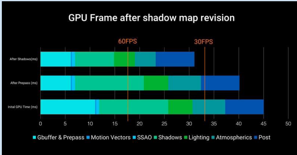
Optimized render at 30 fps
