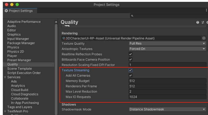
Texture Streaming settings
