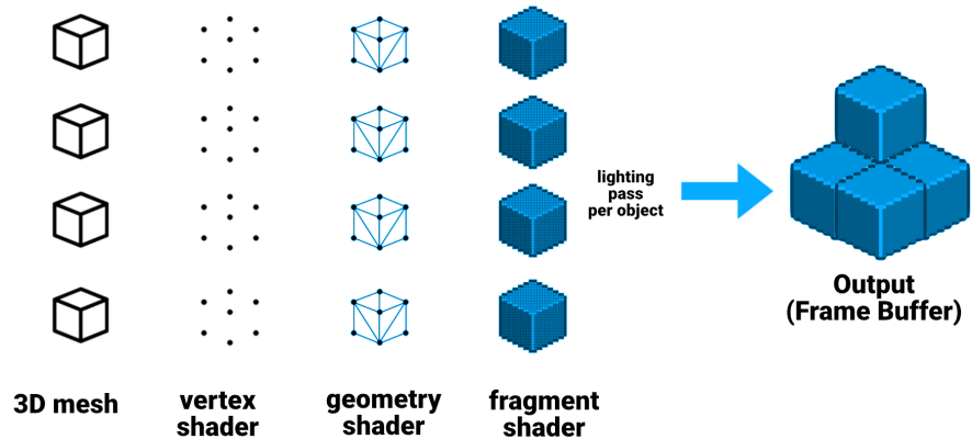
Forward rendering path
