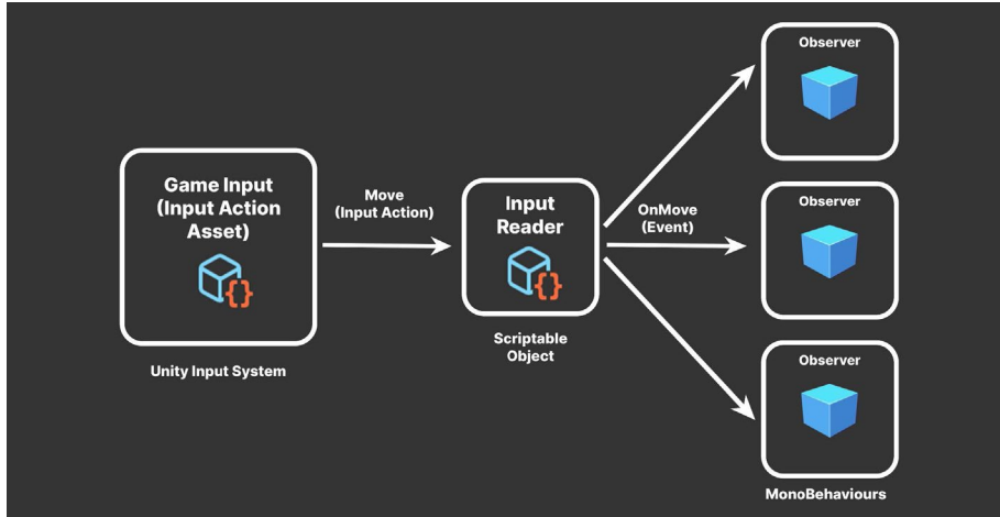
A ScriptableObject InputReader relays events from InputActions.
