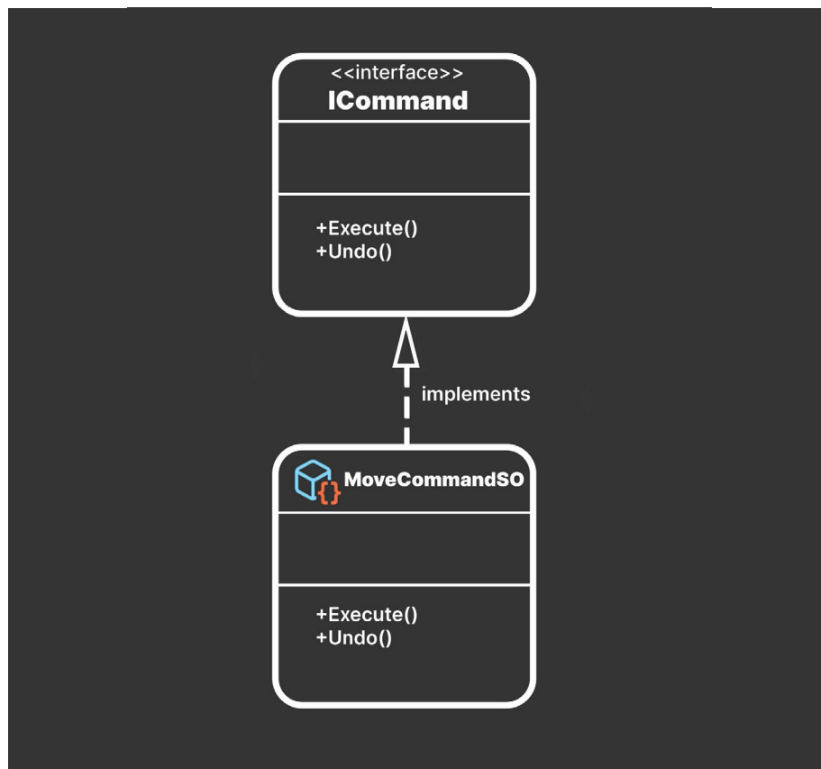
Implementing the command pattern with a ScriptableObject
