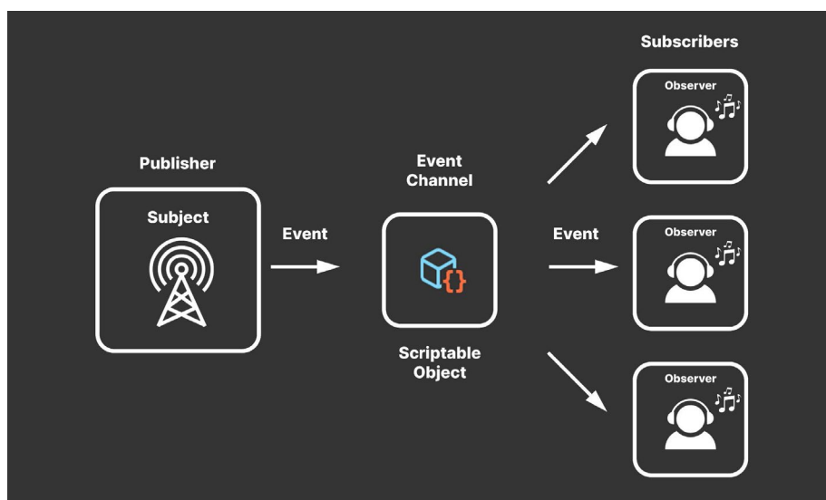
The ScriptableObject-based event channel
