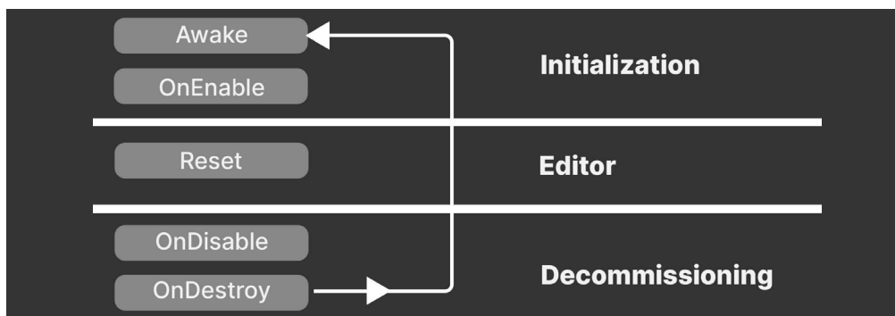
ScriptableObject event functions and execution order
