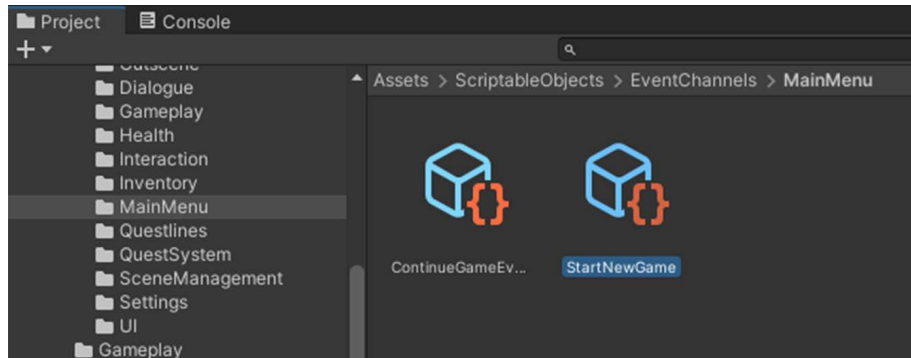
A ScriptableObject-based event, an example of an event channel
