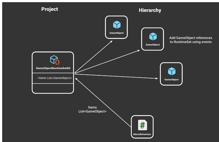
A GameObject Runtime Set
