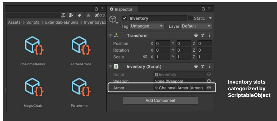
Drag and drop ScriptableObject-based categories
