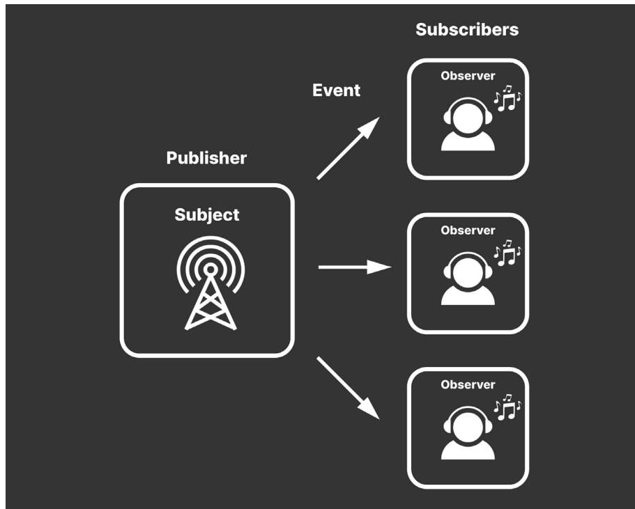
The basic observer pattern
