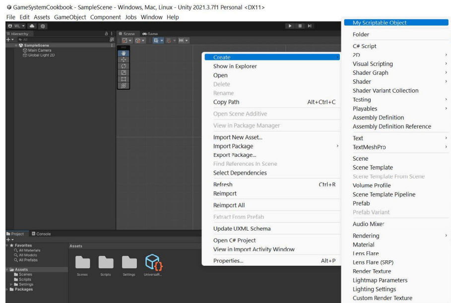
Creating a ScriptableObject
