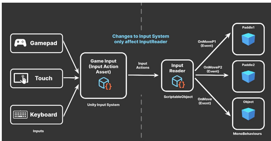
The InputReader insulates objects from direct dependency on the inputs.
