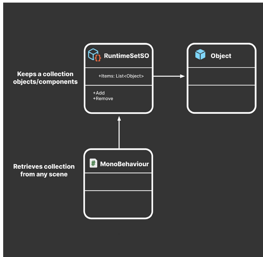
A Runtime Set provides global access to a collection of data.
