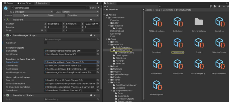
The sample project's Game Manager uses event channels.
