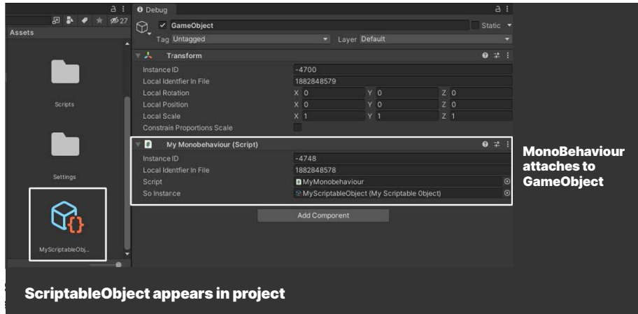
ScriptableObject versus MonoBehaviour
