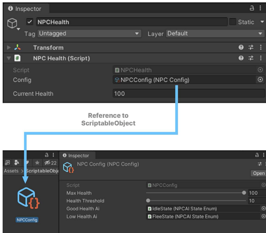
Refactoring splits data between a MonoBehaviour and ScriptableObject
