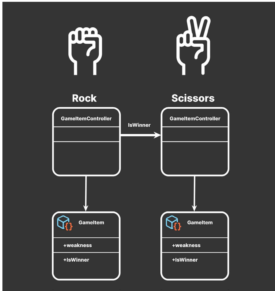
ScriptableObjects with comparison logic Source: Flaticon
