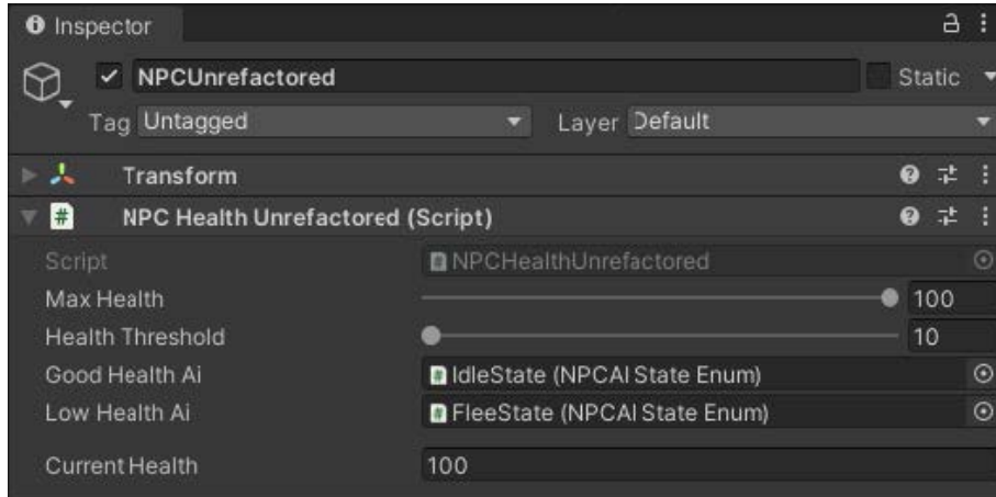
An NPCHealth MonoBehaviour before refactoring
