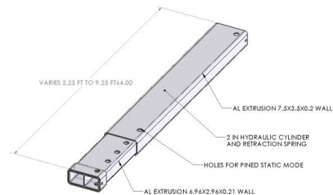
2 IN HYDRAULIC STRUT
