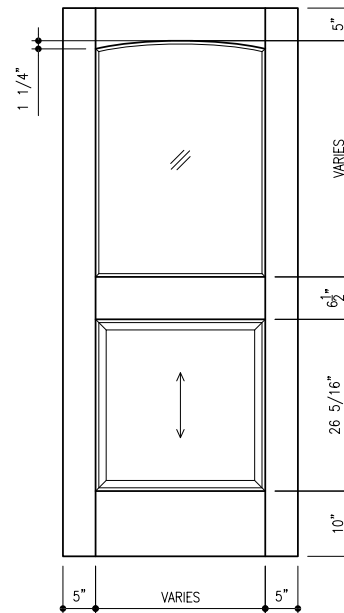
702 Standard Archtop Series 1 Panel 1 Lite – Interior
