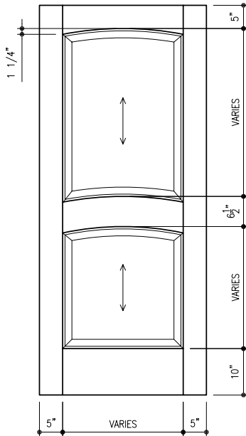
702 Modified Standard Archtop Series 2 Panel w/ Shaped Lock Rail – Interior
