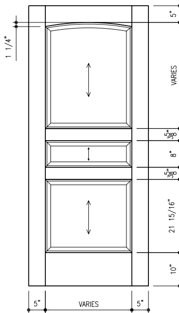
703 Standard Archtop Series 3 Panel – Interior
