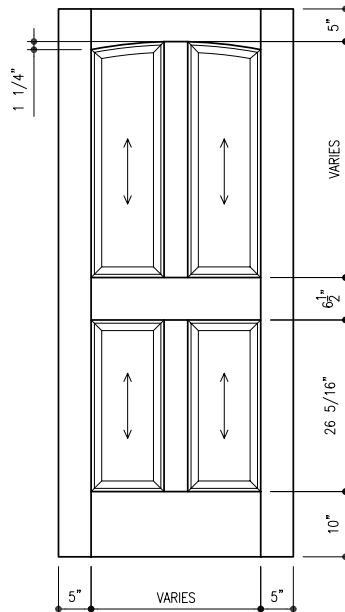
704 Standard Archtop Series 4 Panel – Interior
