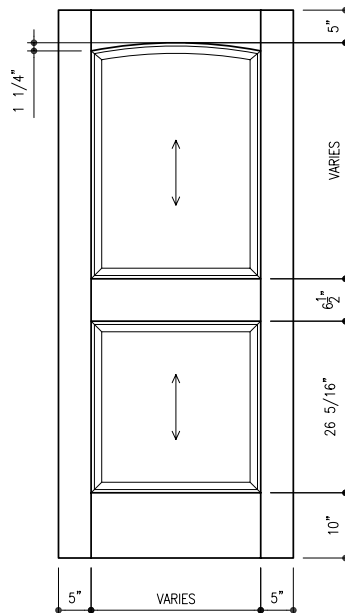
702 Standard Archtop Series 2 Panel – Interior
