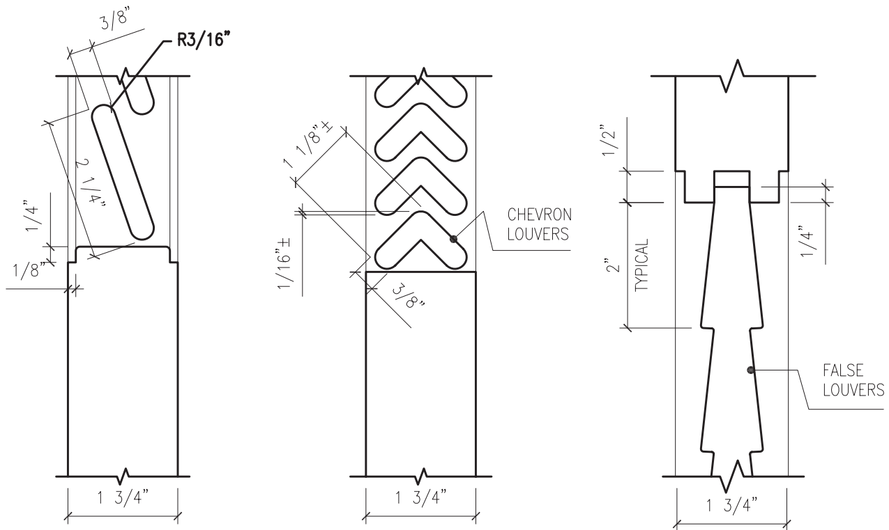
STANDARD LOUVER
