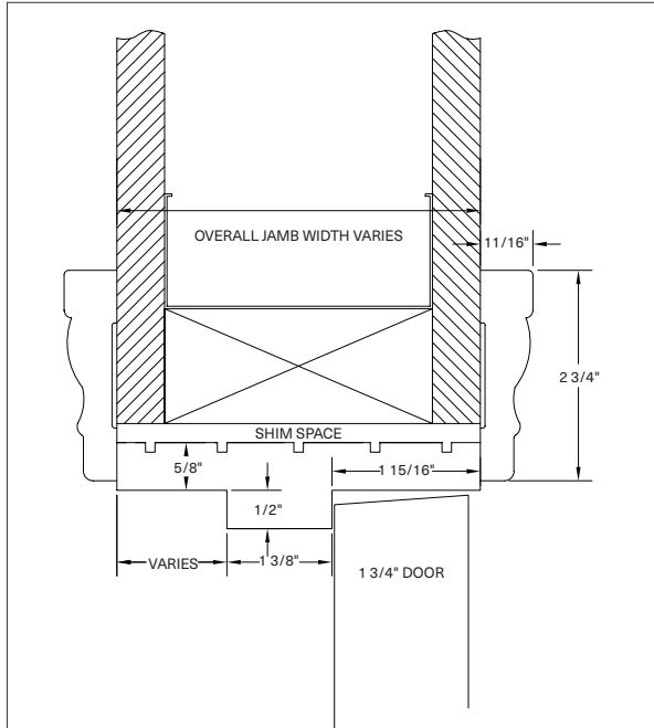
Standard Double Rabbet Jamb with Colonial Casing
