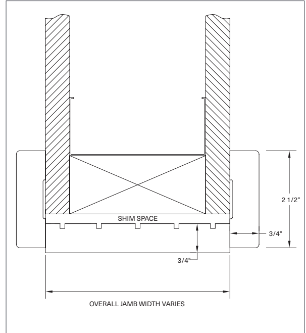
Standard No Stop Jamb with Contemporary Casing
