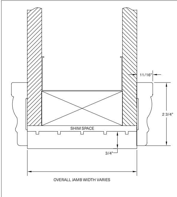
Standard No Stop Jamb with Colonial Casing
