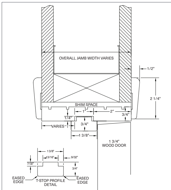
Standard T-Stop Jamb with Sleek Casing
