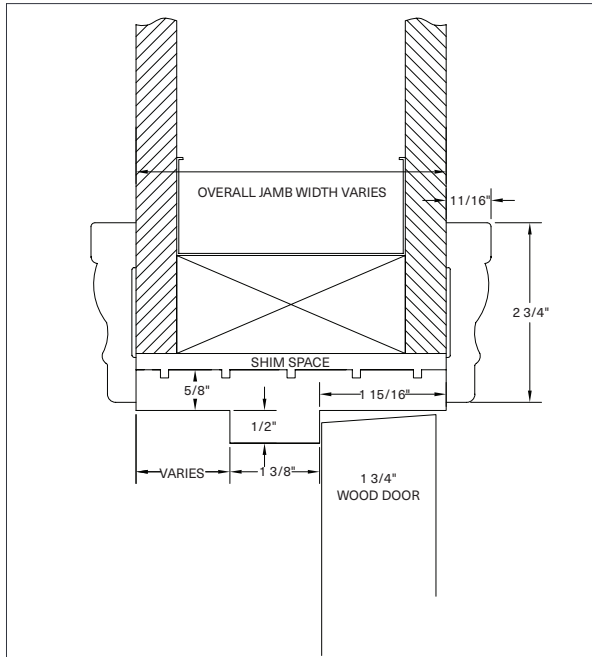
Standard T-Stop Jamb with Colonial Casing
