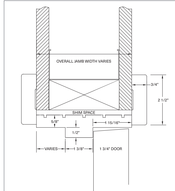
Standard Double Rabbet Jamb with Contemporary Casing
