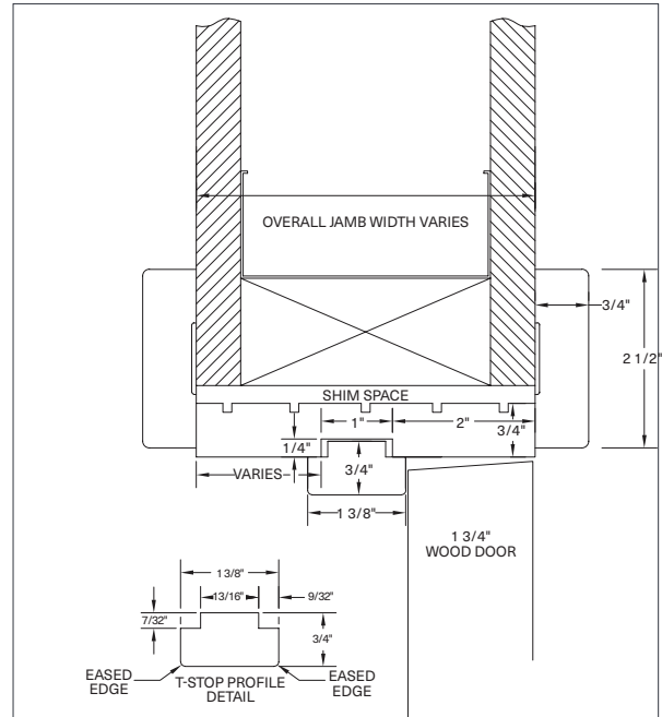
Standard T-Stop Jamb with Contemporary Casing
