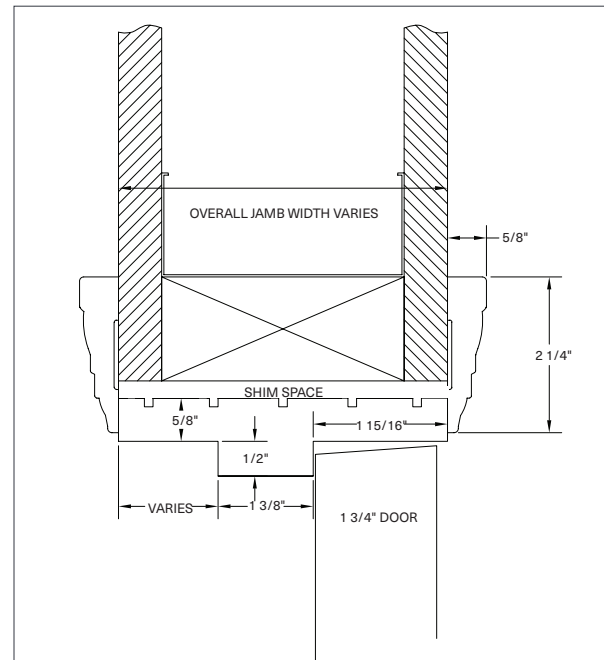
Standard Double Rabbet Jamb with Traditional Casing
