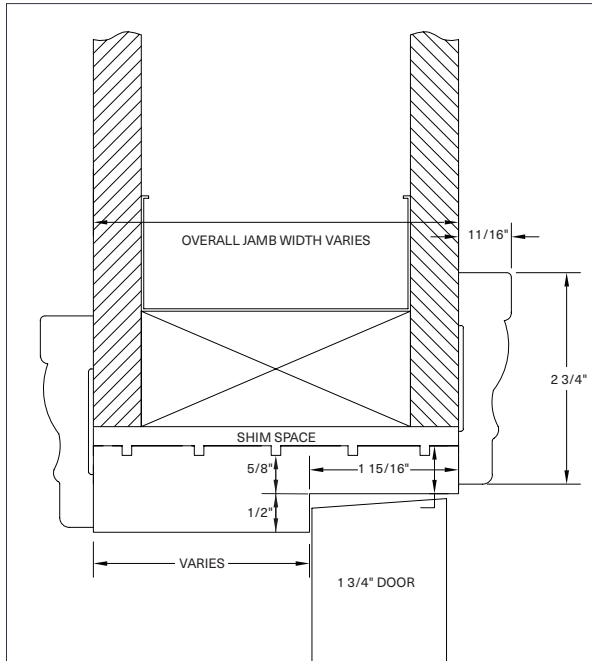
Standard Single Rabbet Jamb with Colonial Casing
