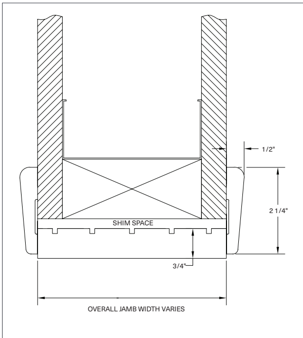
Standard No Stop Jamb with Sleek Casing
