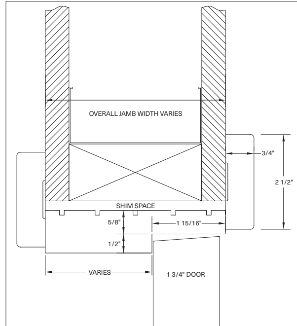
Standard Single Rabbet Jamb with Contemporary Casing
