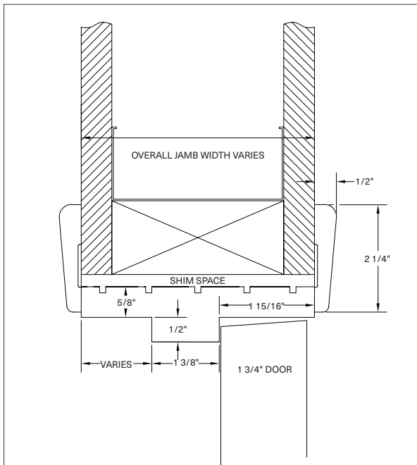
Standard Double Rabbet Jamb with Sleek Casing
