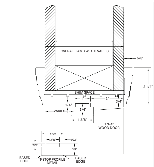
Standard T-Stop Jamb with Traditional Casing
