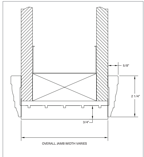
Standard No Stop Jamb with Traditional Casing
