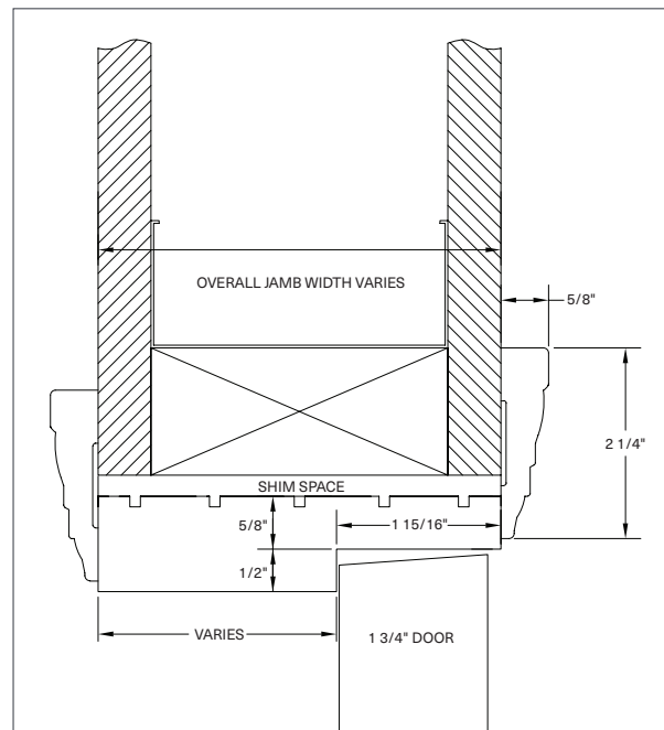
Standard Single Rabbet Jamb with Traditional Casing
