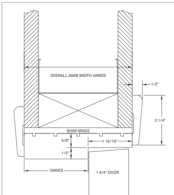
Standard Single Rabbet Jamb with Sleek Casing
