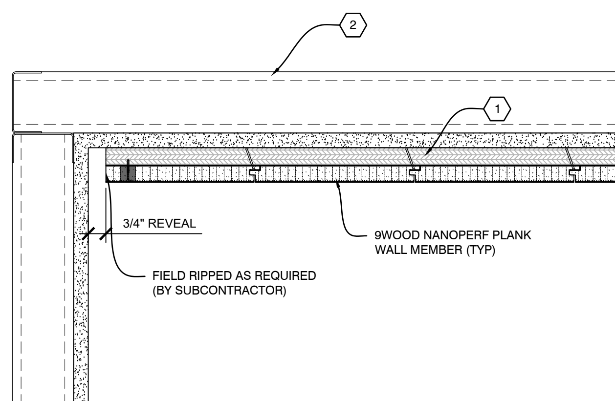
A1 PLAN VIEW - PERIMETER SCALE: 1/4" = 1"
