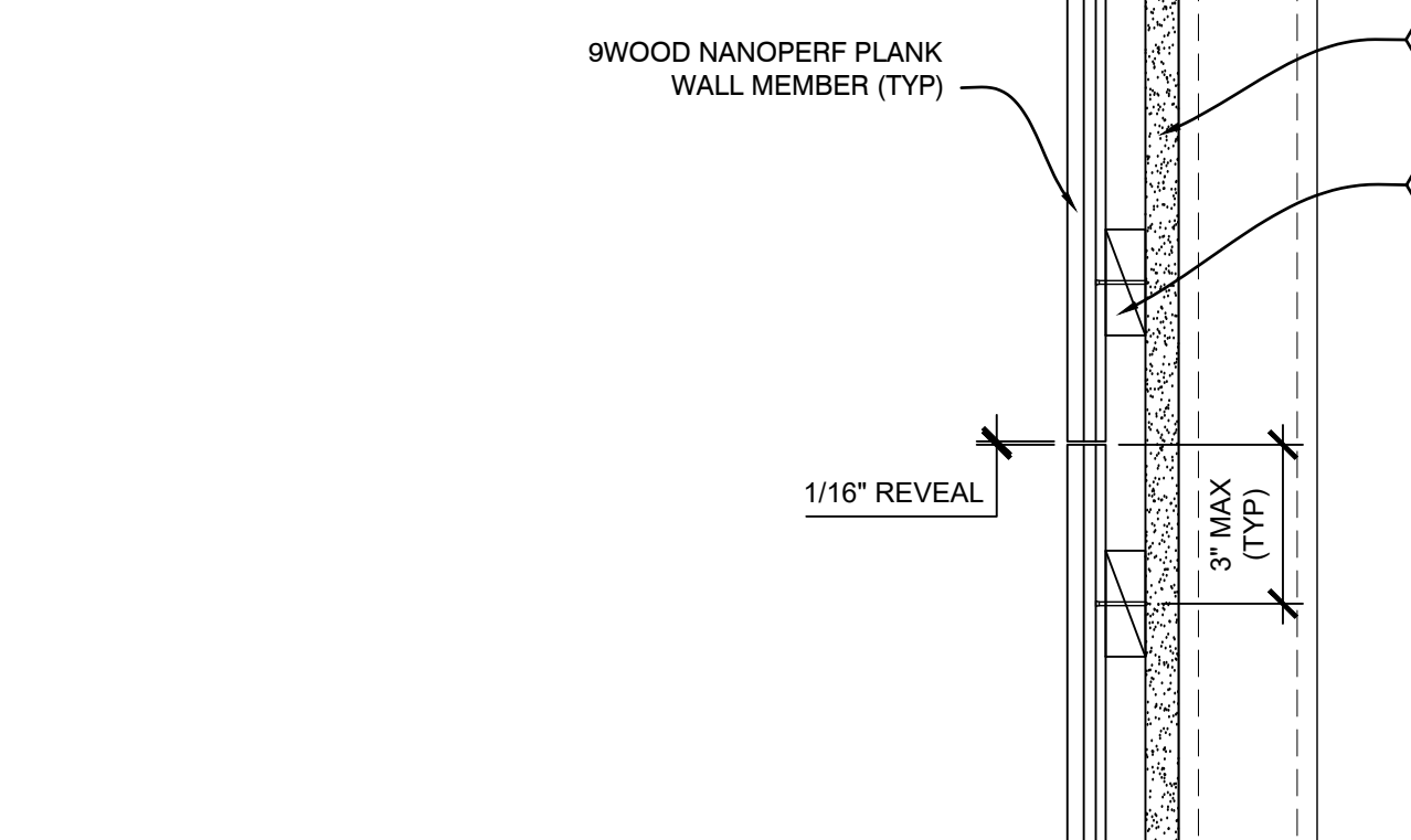
B4 SECTION - ABUTTING REVEAL SCALE: 1/4" = 1"
