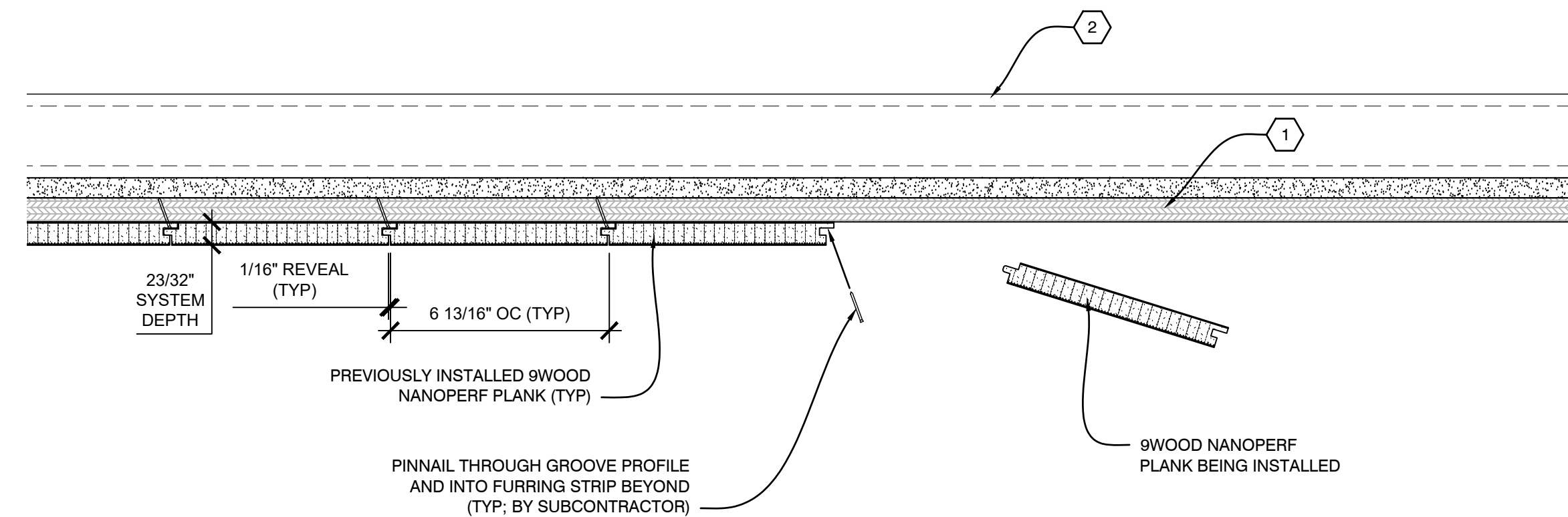
B2 INSTALLATION PROCESS - NANOPERF PLANK WALL SYSTEM SCALE: 1/4" = 1"
