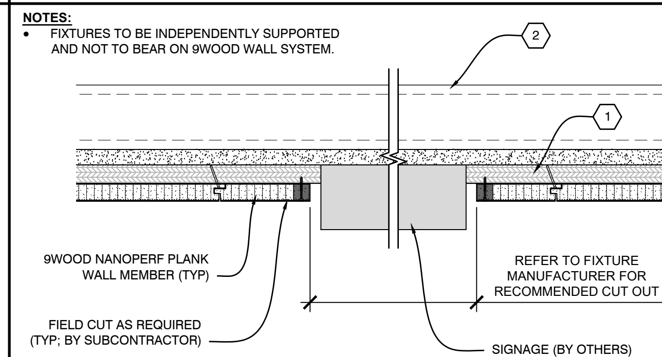
B2 INSTALLATION PROCESS - NANOPERF PLANK WALL SYSTEM SCALE: 1/4" = 1"
