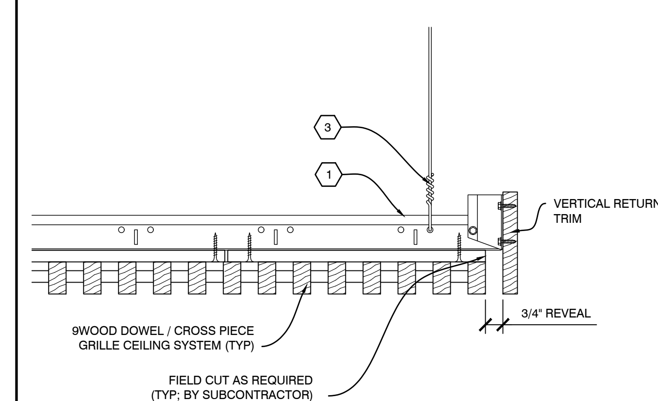
B4 SECTION - PERIMETER SCALE: 1/4" = 1'
