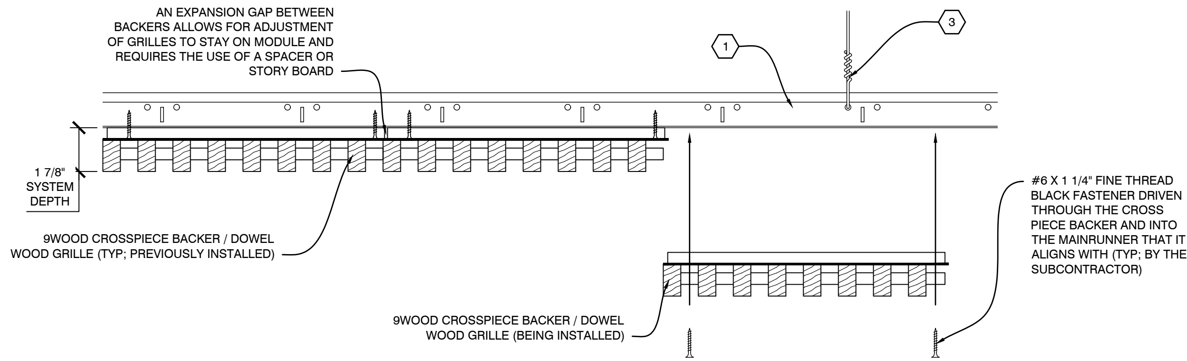
C1 INSTALLATION PROCESS - CROSS PIECE BACKER WOOD GRILLE SCALE: 1/4" = 1"
