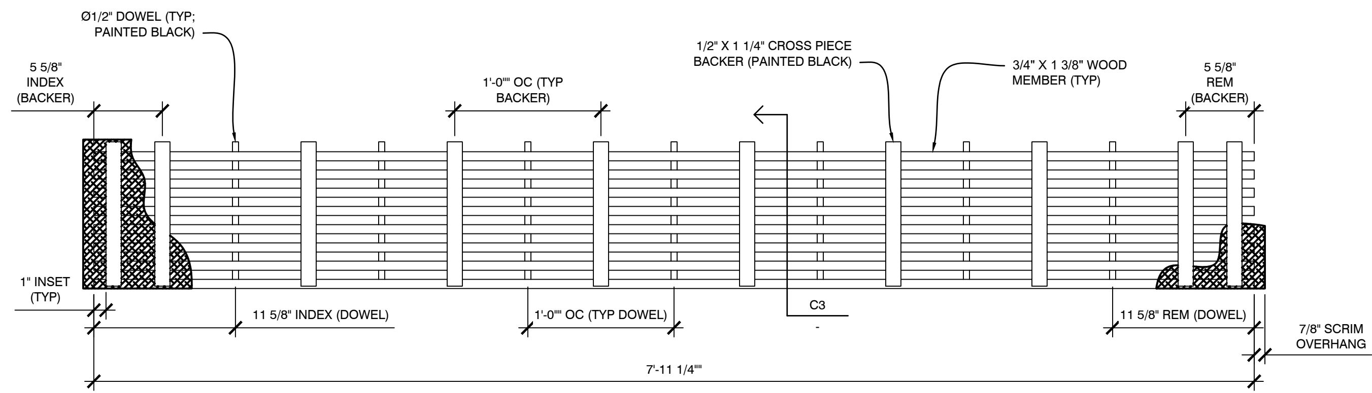
D3 PLAN VIEW - CROSS PIECE BACKER WOOD GRILLE SCALE: 1 1/2" = 1"
