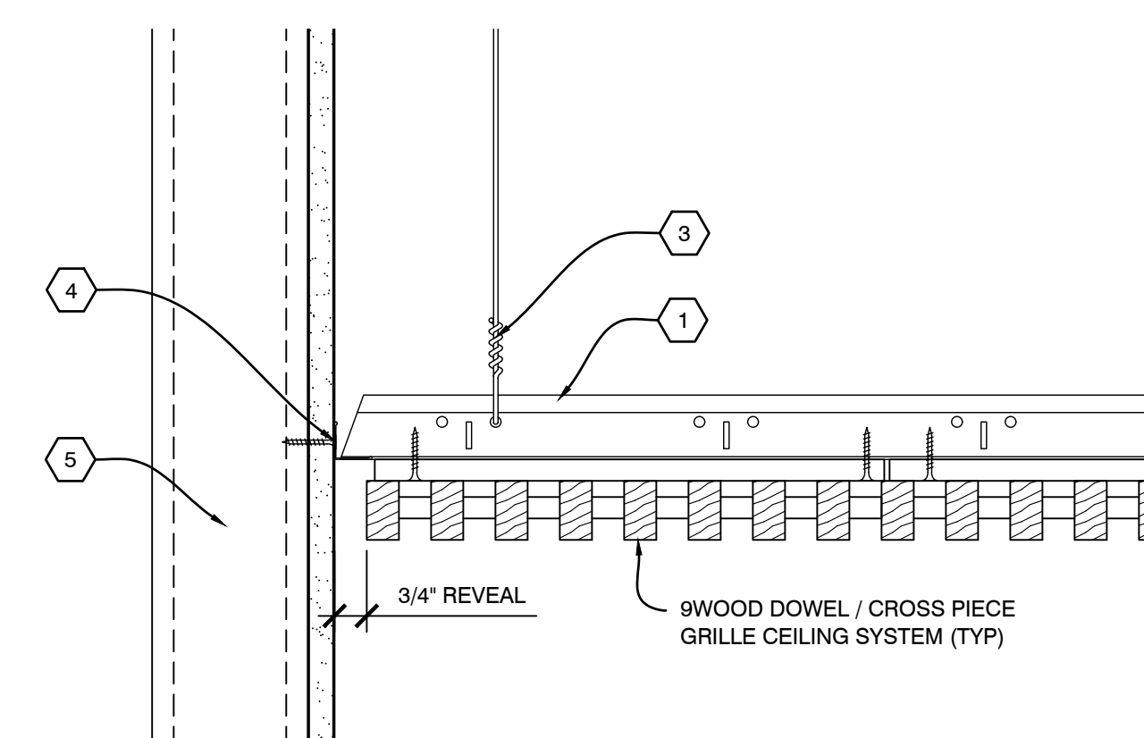
B1 SECTION - PERIMETER SCALE: 1/4" = 1'
