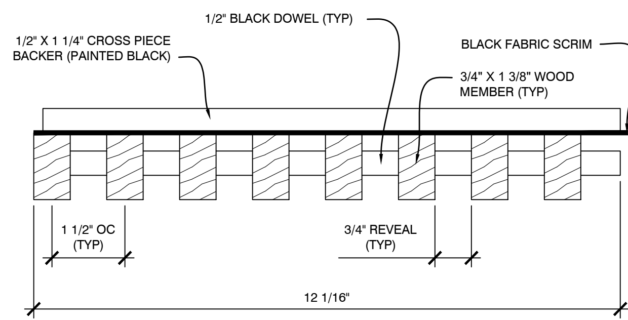
C3 SECTION - CROSS PIECE BACKER WOOD GRILLE SCALE: 1/2" = 1"
