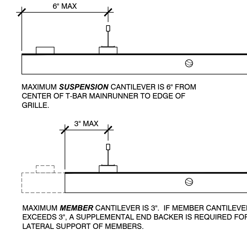
C4 SECTION - CANTILEVER RULES SCALE: 1/4" = 1"
