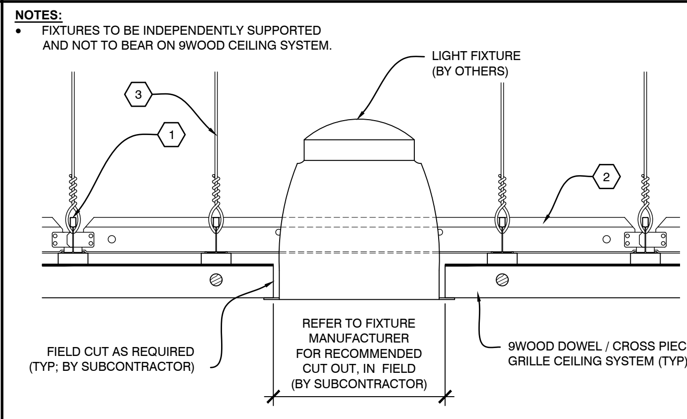
A2 SECTION - LIGHT FIXTURE SCALE: 1/4" = 1"
