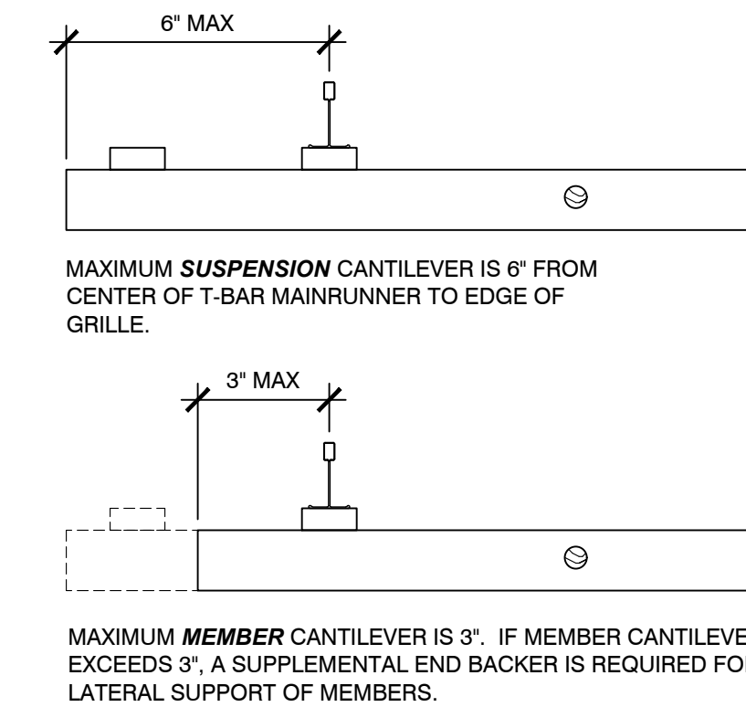
C4 SECTION - CANTILEVER RULES SCALE: 1/4" = 1'
