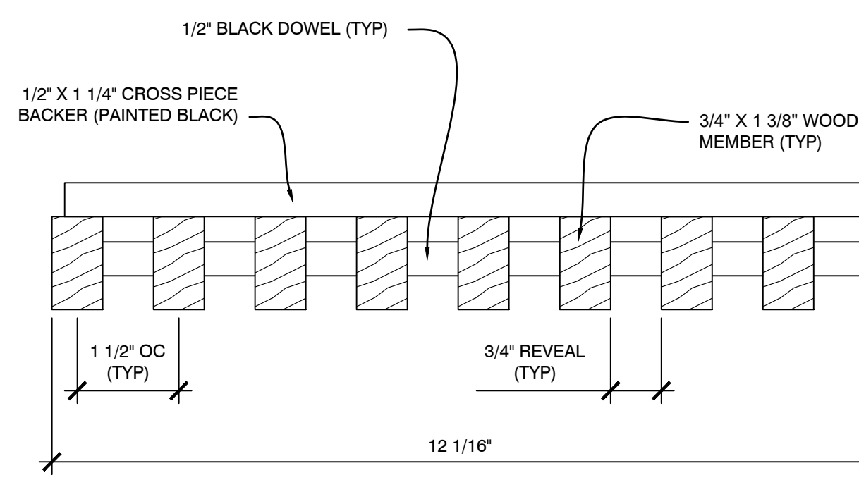
C3 SECTION - CROSS PIECE BACKER WOOD GRILLE SCALE: 1/2" = 1'
