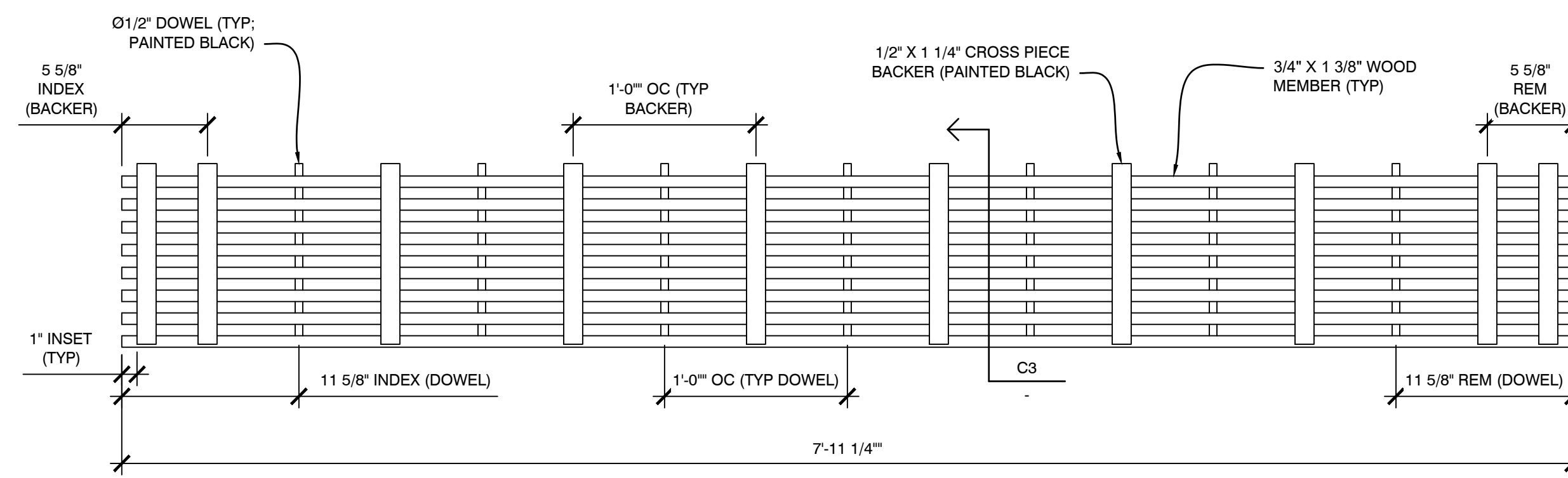
D3 PLAN VIEW - CROSS PIECE BACKER WOOD GRILLE SCALE: 1 1/2" = 1'
