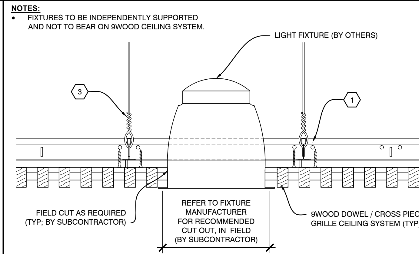
B2 SECTION - LIGHT FIXTURE SCALE: 1/4" = 1'
