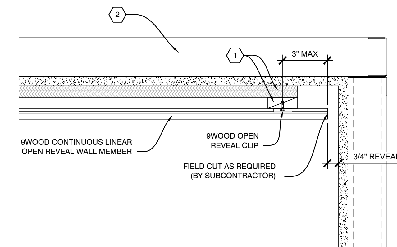
A4 PLAN VIEW - PERIMETER SCALE: 1/4" = 1"
