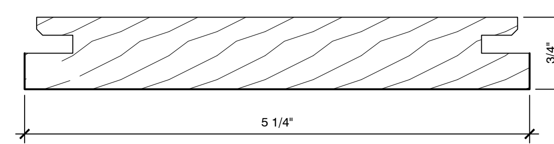
D4 SECTION - CONTINUOUS LINEAR OPEN REVEAL MEMBER SCALE: 1" = 1"
