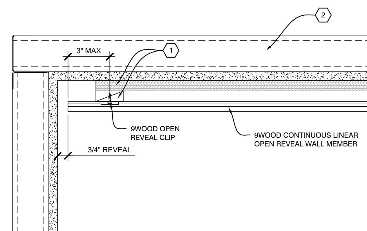
A1 PLAN VIEW - PERIMETER SCALE: 1/4" = 1"
