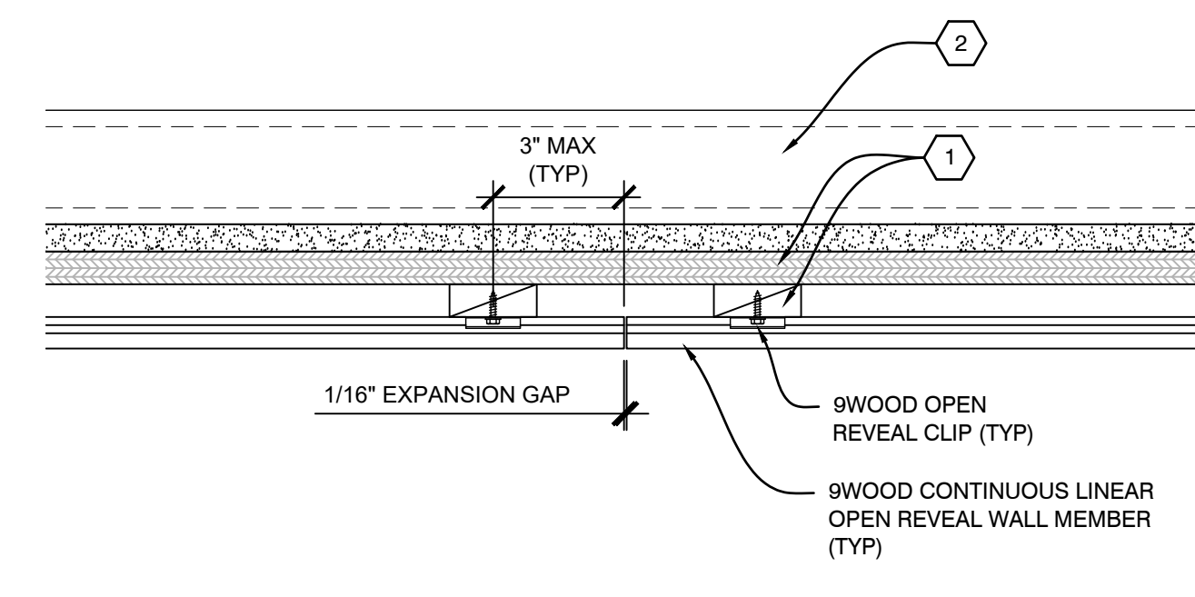
A3 PLAN VIEW - ABUTTING REVEAL SCALE: 1/4" = 1"
