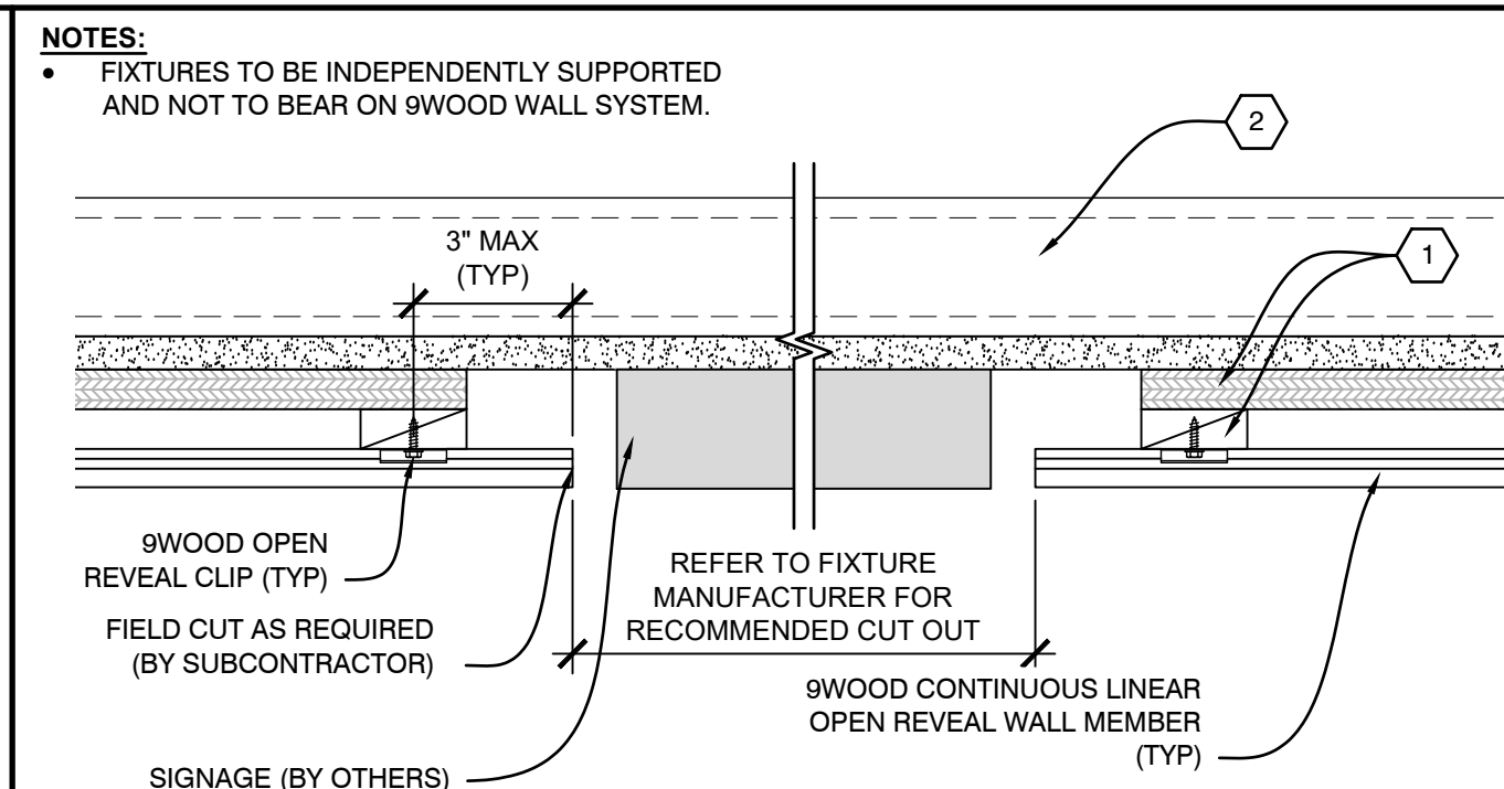
A2 PLAN VIEW - WALL PENETRATION SCALE: 1/4" = 1"
