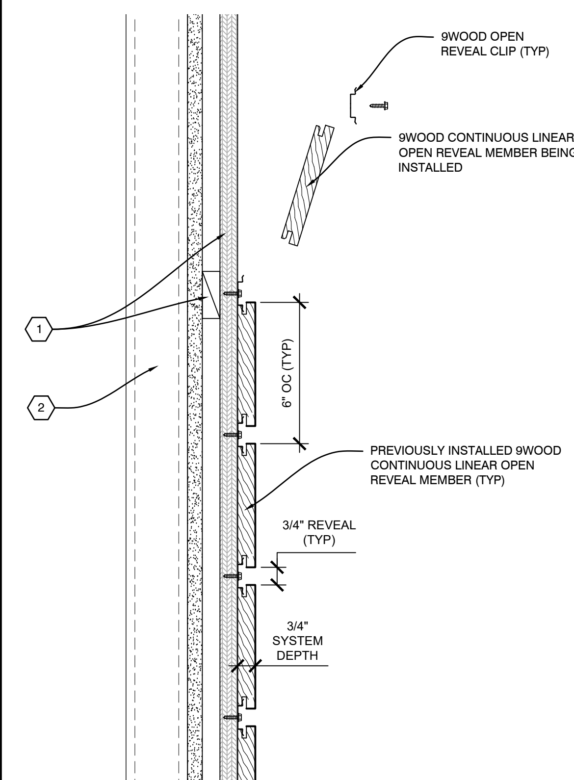
B3 INSTALLATION PROCESS - CONTINUOUS LINEAR OPEN REVEAL MEMBER SCALE: 1/4" = 1"
