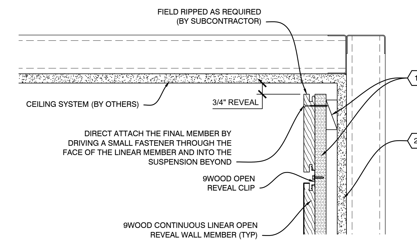
D4 SECTION - CEILING PERIMETER SCALE: 1/4" = 1"
