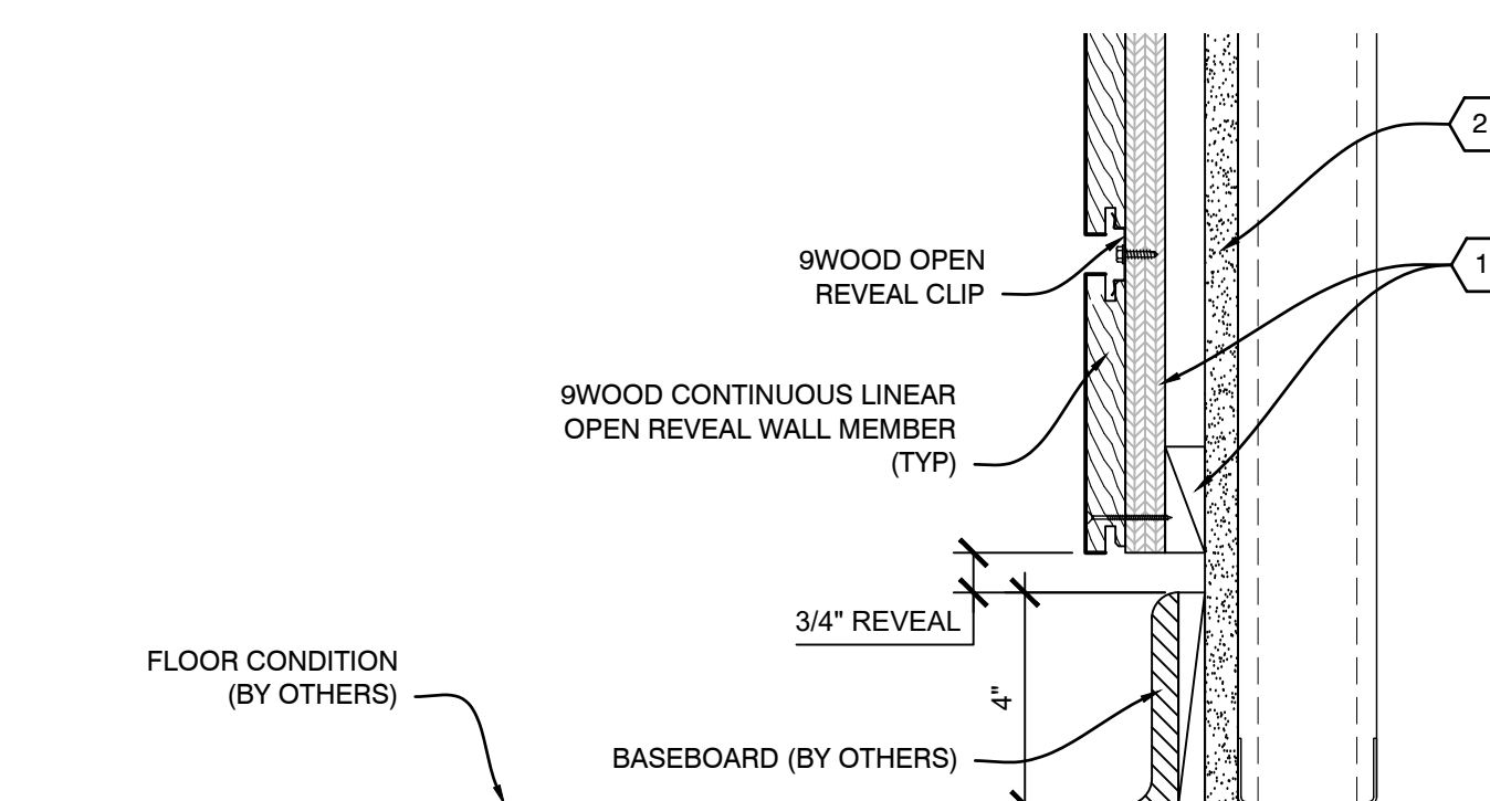
B4 SECTION - FLOOR PERIMETER SCALE: 1/4" = 1"
