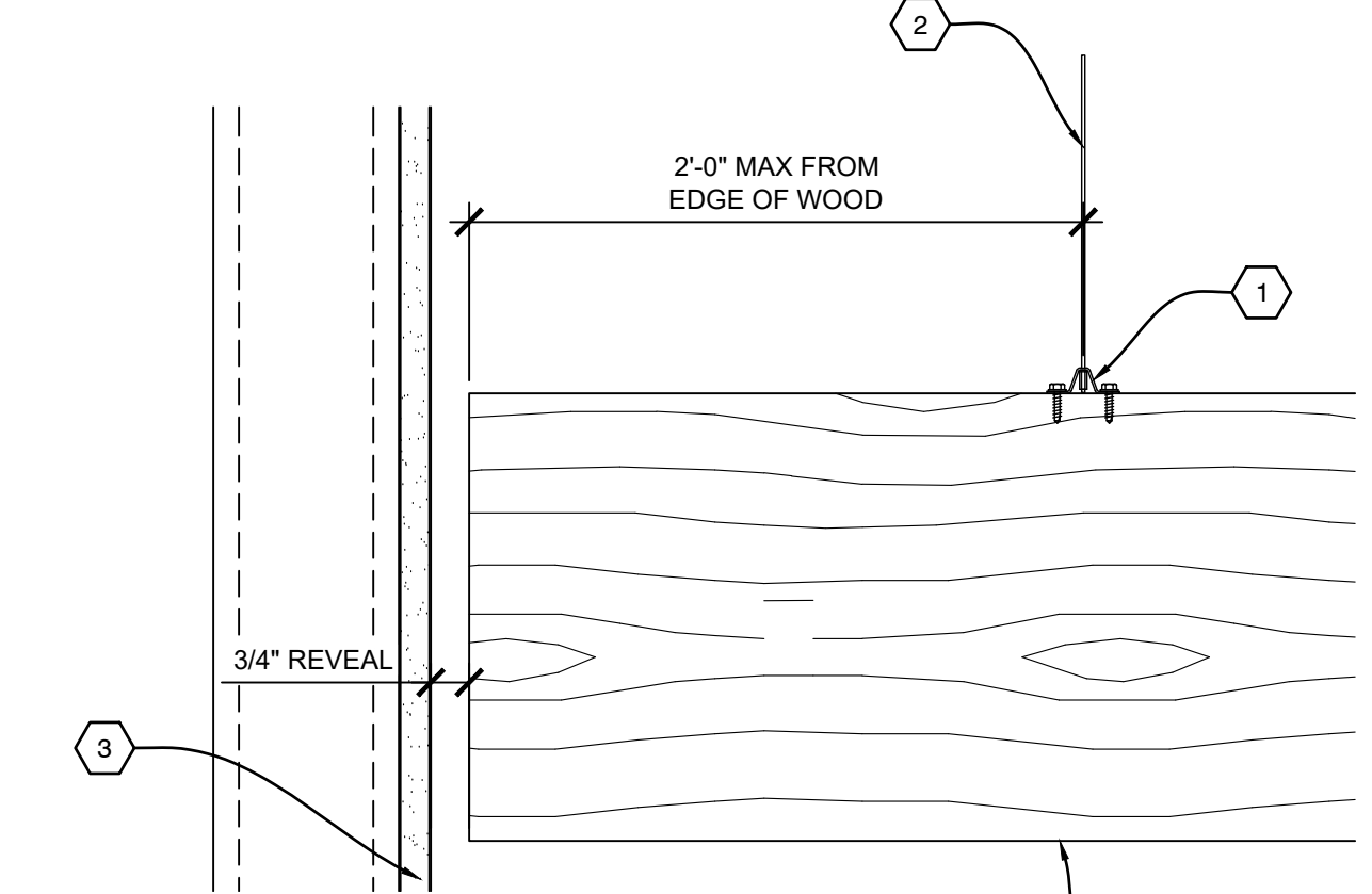
B3 SECTION - PERIMETER SCALE: 1/4" = 1'
