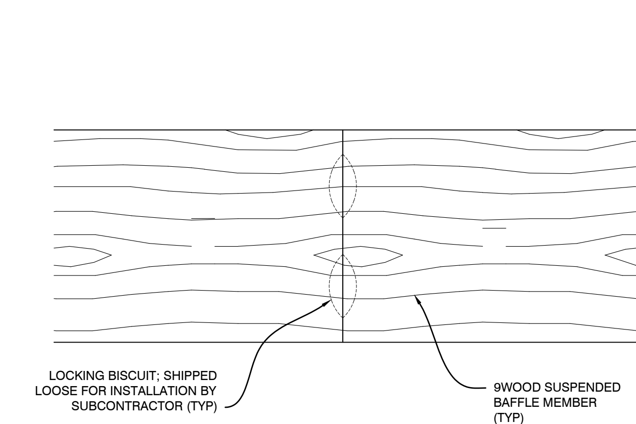
B1 SECTION - ABUTTING MEMBERS SCALE: 1/4" = 1'
