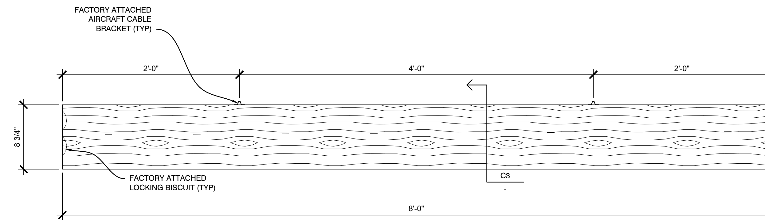
D3 SIDE VIEW - WOOD BAFFLE "1.8" SCALE: 1 1/2" = 1'
