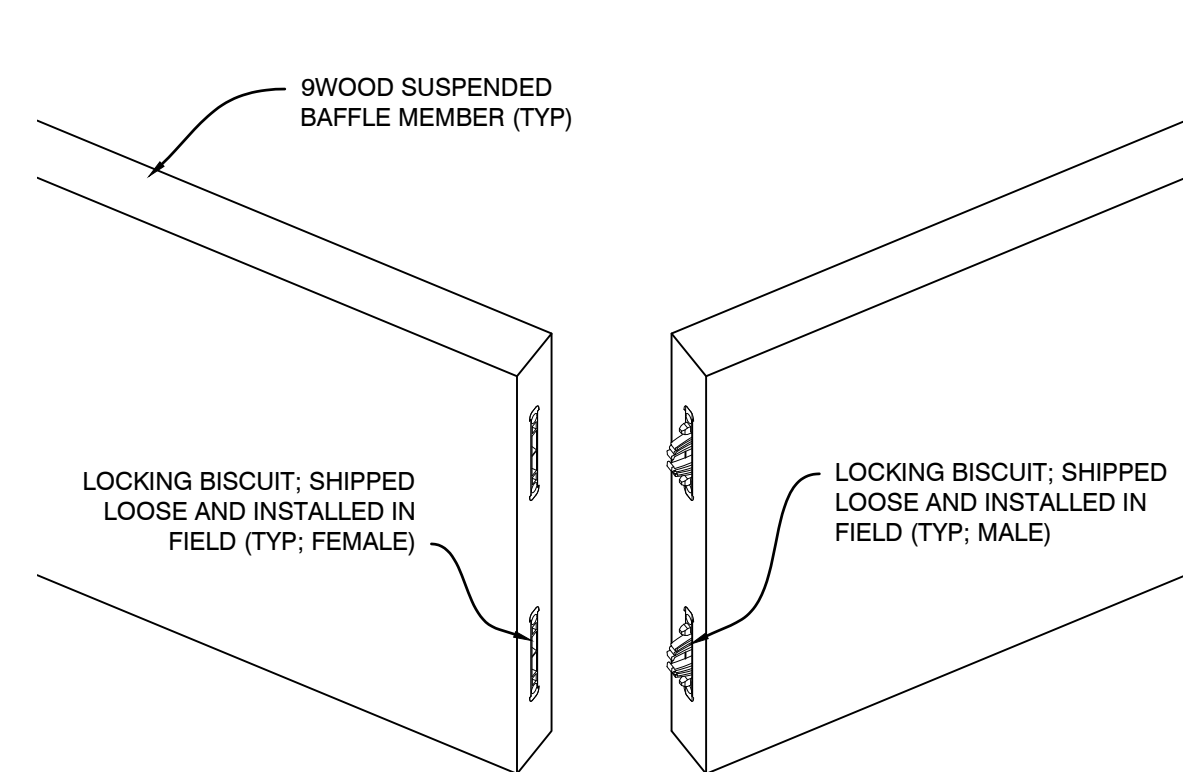
C2 DETAIL - LOCKING BISCUIT JOINT SCALE: 1/2" = 1'
