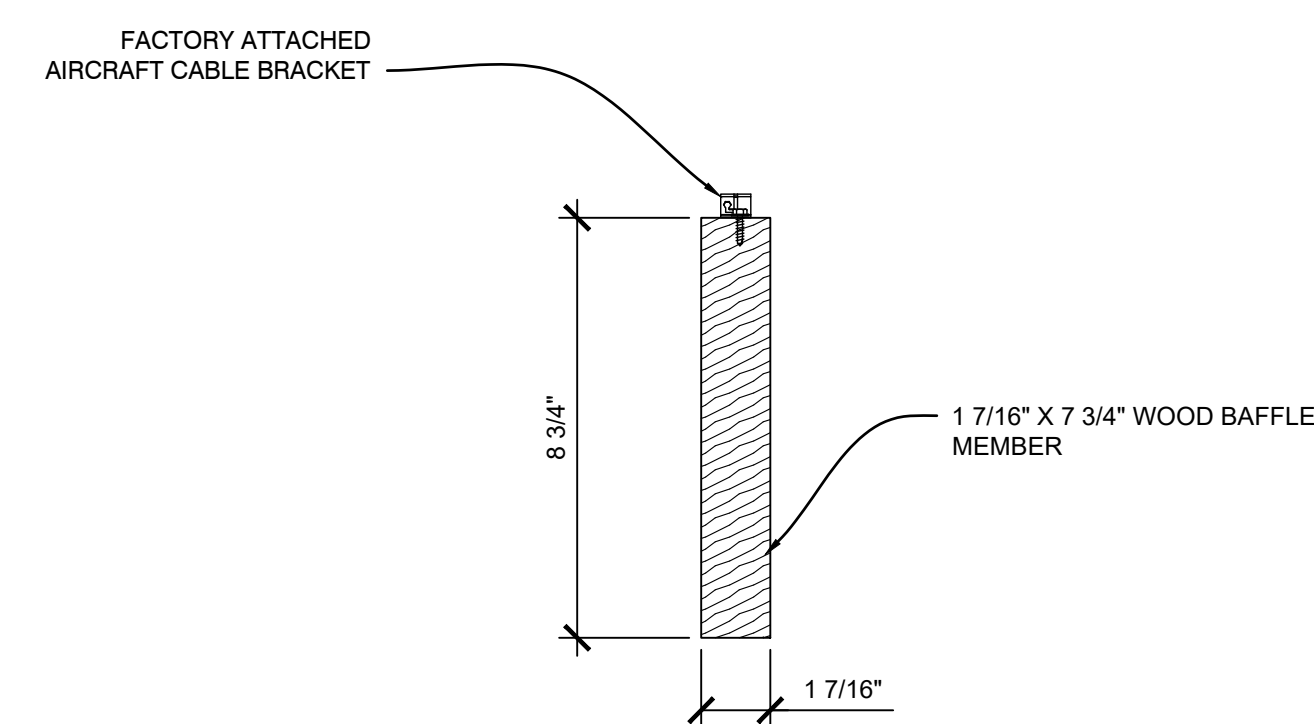
B2 SECTION - WOOD BAFFLE SCALE: 1/4" = 1'
