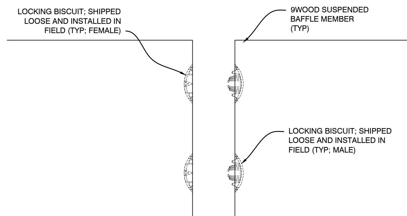
C1 DETAIL - LOCKING BISCUIT JOINT SCALE: 1/2" = 1'
