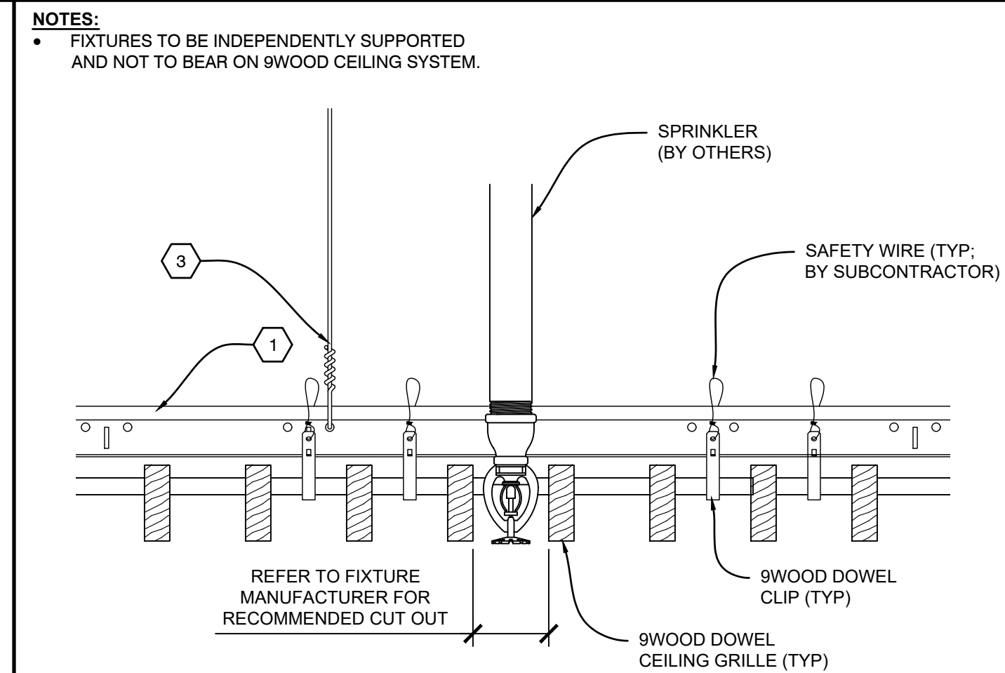
C3 INSTALLATION PROCESS - DOWEL CEILING GRILLE SCALE: 1/4" = 1'
