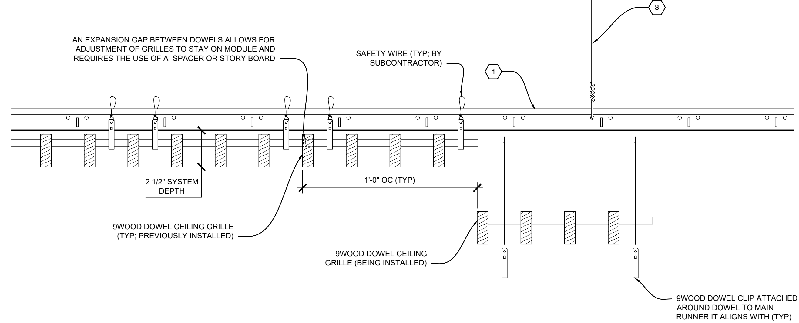
C3 INSTALLATION PROCESS - DOWEL CEILING GRILLE SCALE: 1/4" = 1'
