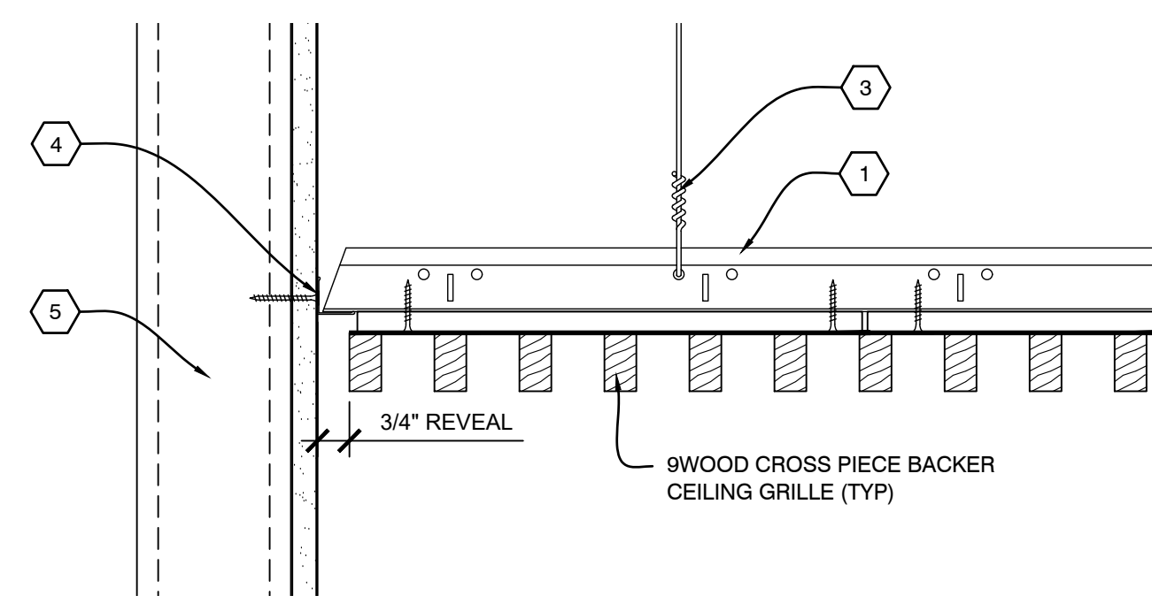
B1 SECTION - PERIMETER SCALE: 1/4" = 1'
