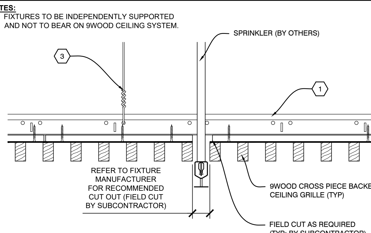
B3 SECTION - SPRINKLER SCALE: 1/4" = 1'
