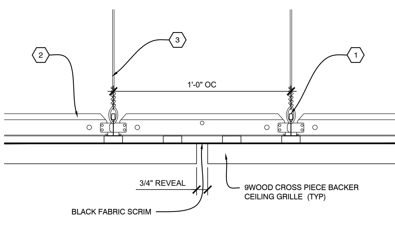
A3 SECTION - ABUTTING REVEAL SCALE: 1/4" = 1'
