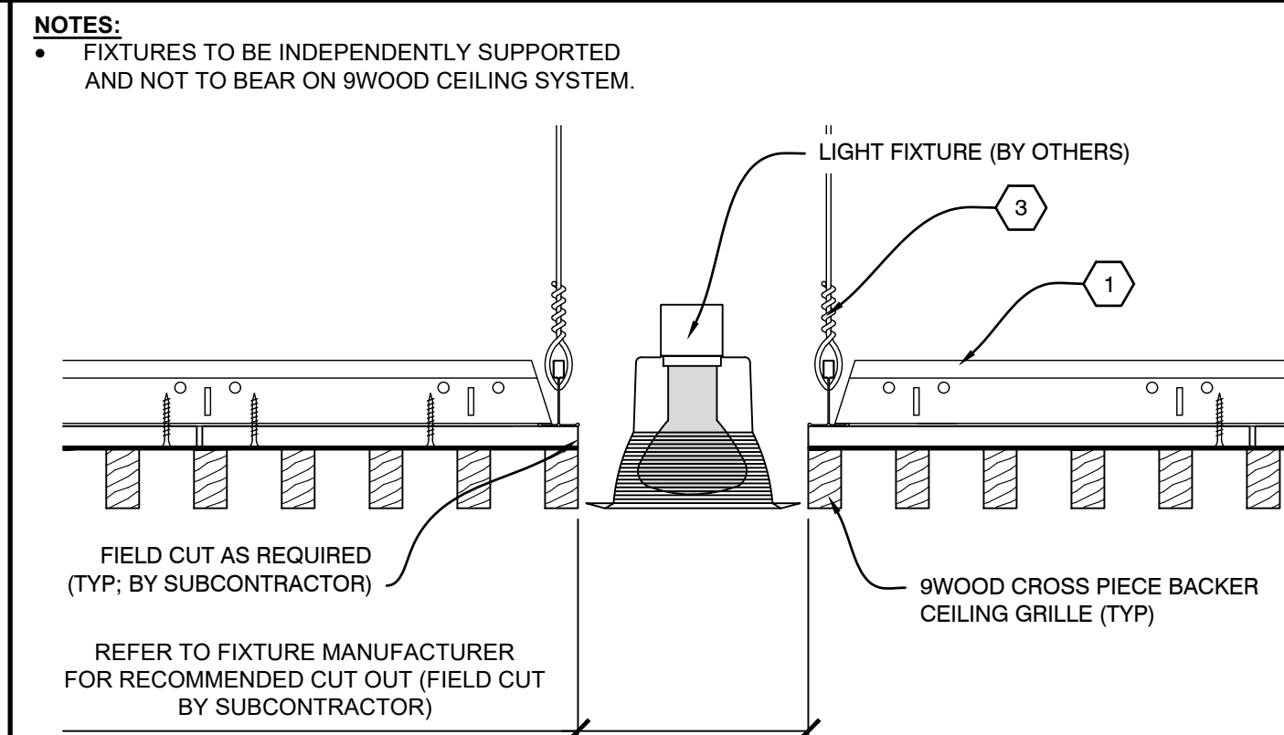
B2 SECTION - LIGHT FIXTURE SCALE: 1/4" = 1'
