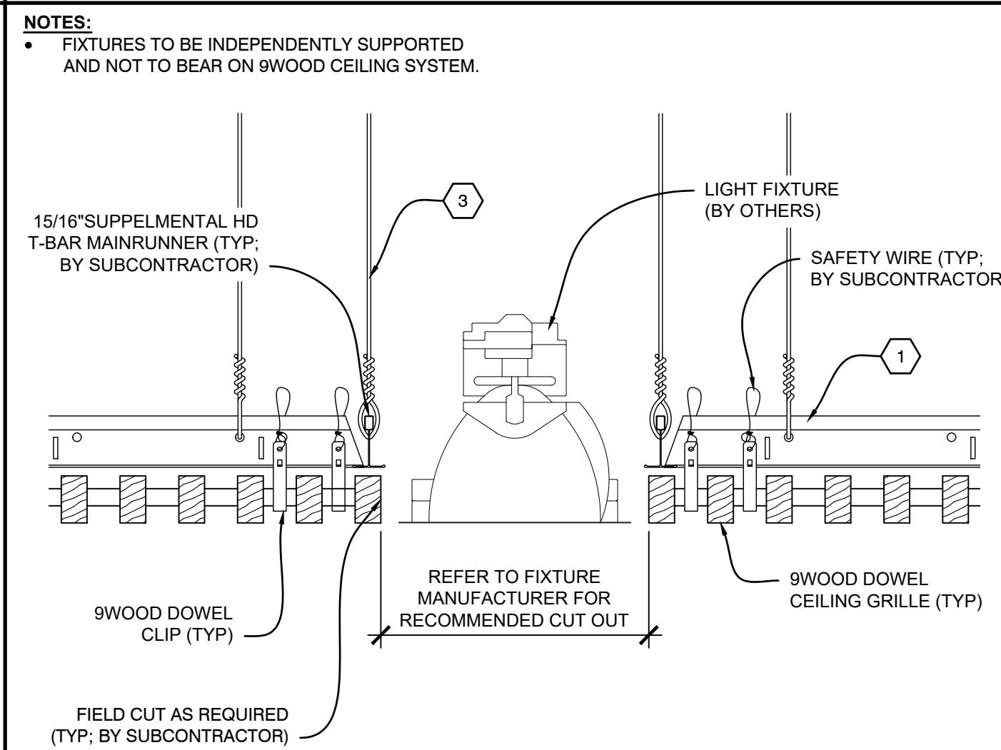
C3 INSTALLATION PROCESS - DOWEL CEILING GRILLE SCALE: 1/4" = 1'
