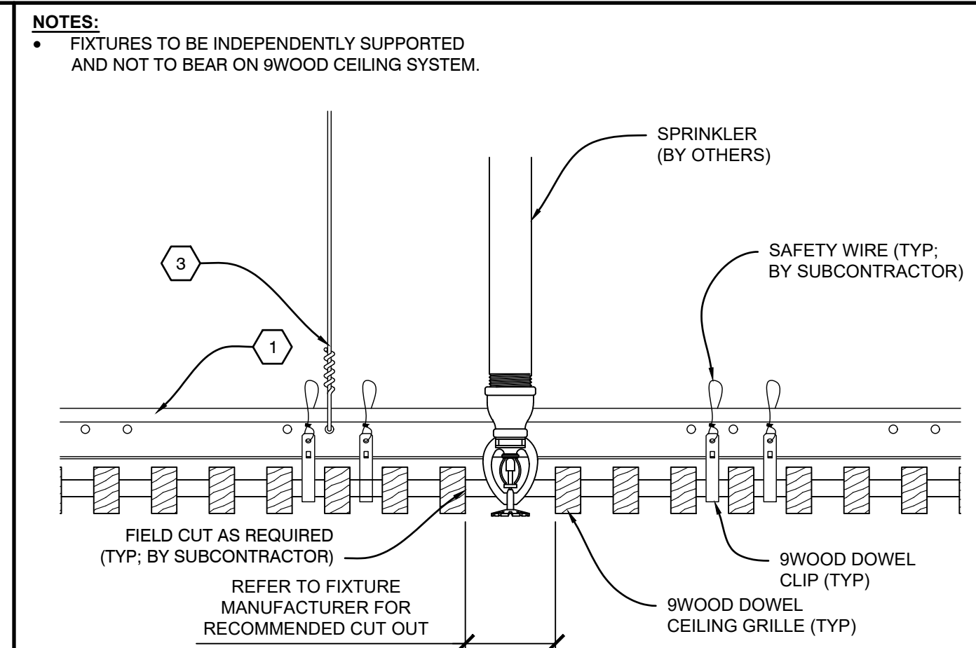
C3 INSTALLATION PROCESS - DOWEL CEILING GRILLE SCALE: 1/4" = 1'
