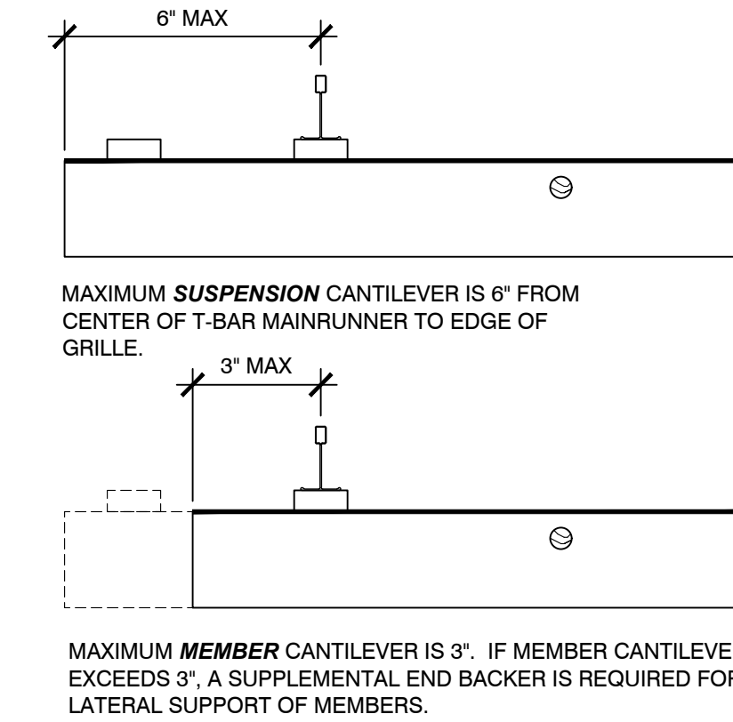
C4 SECTION - CANTILEVER RULES SCALE: 1/4" = 1'
