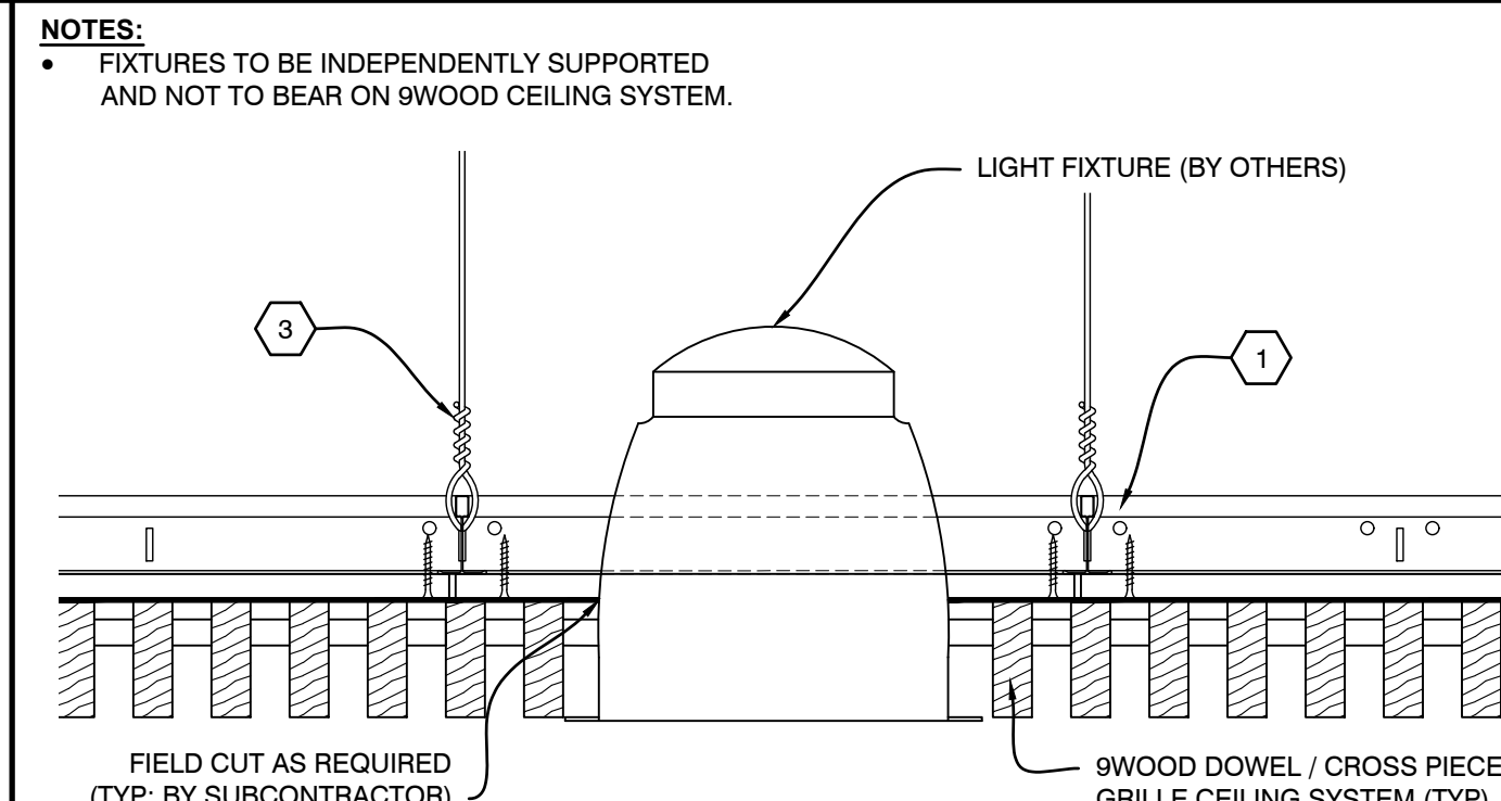
C1 INSTALLATION PROCESS - CROSS PIECE BACKER WOOD GRILLE SCALE: 1/4" = 1"
