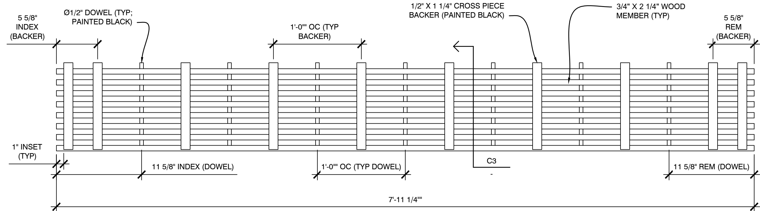
D3 PLAN VIEW - CROSS PIECE BACKER WOOD GRILLE SCALE: 1 1/2" = 1"
