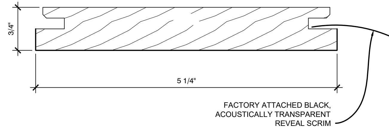
C3 SECTION - CONTINUOUS LINEAR MEMBER SCALE: 1" = 1"
