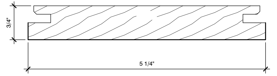
C3 SECTION - CONTINUOUS LINEAR MEMBER SCALE: 1" = 1"
