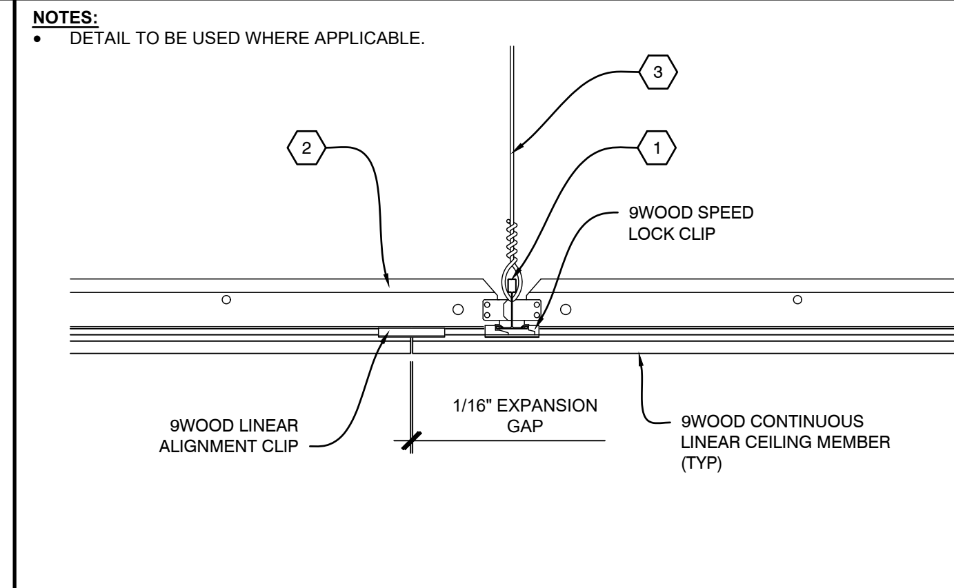
A3 SECTION - ABUTTING MEMBERS SCALE: 1/4" = 1"
