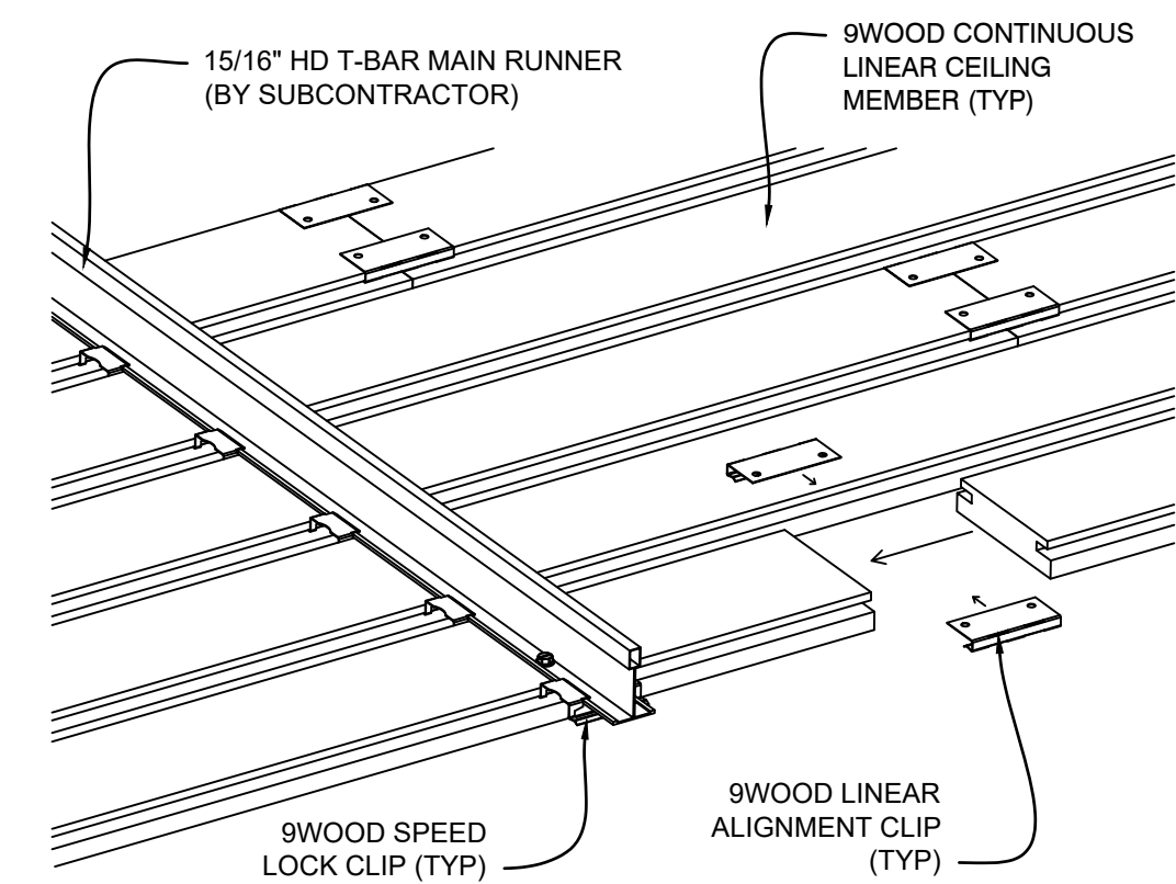
C4 ISO VIEW - INSTALLATION SCALE: NOT TO SCALE
