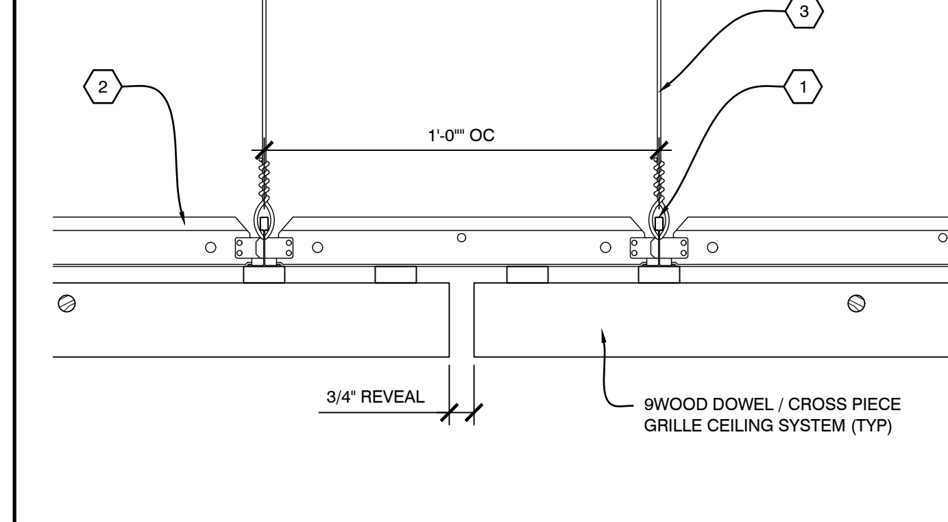
A3 SECTION - ABUTTING REVEAL SCALE: 1/4" = 1"
