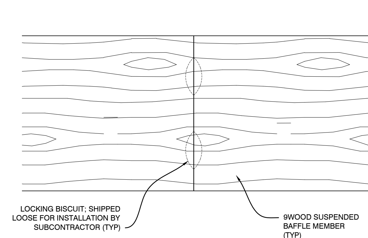
B1 SECTION - ABUTTING MEMBERS SCALE: 1/4" = 1"
