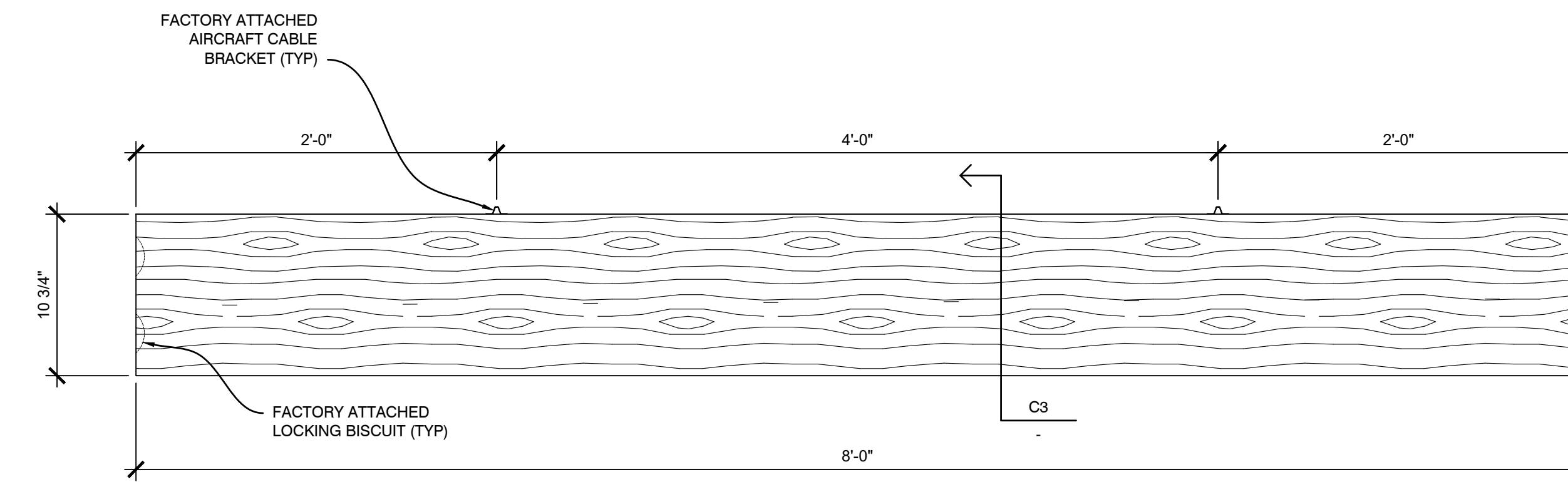
D3 SIDE VIEW - WOOD BAFFLE "1.8" SCALE: 1 1/2" = 1"
