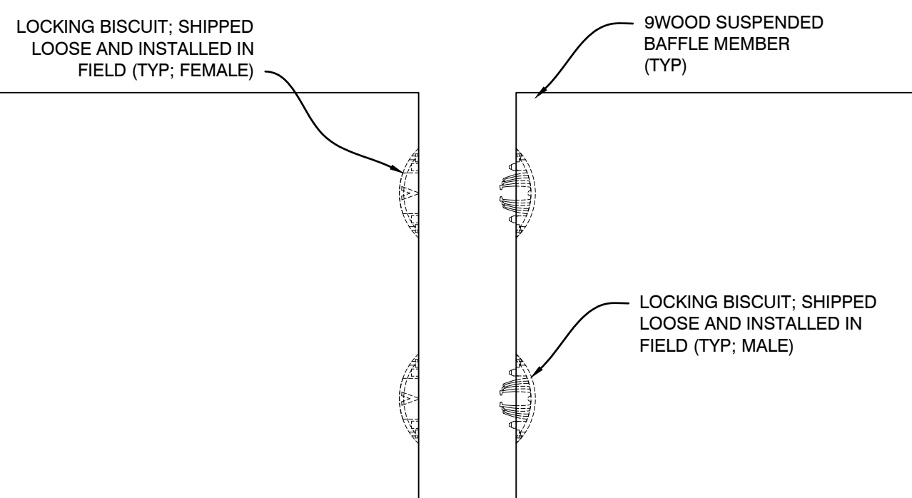
C1 DETAIL - LOCKING BISCUIT JOINT SCALE: 1/2" = 1"
