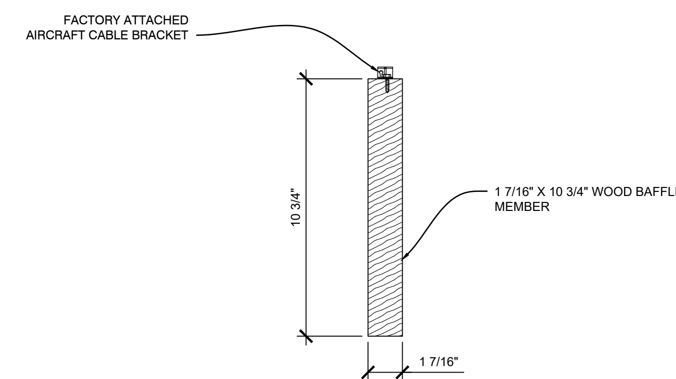
B2 SECTION - WOOD BAFFLE SCALE: 1/4" = 1"
