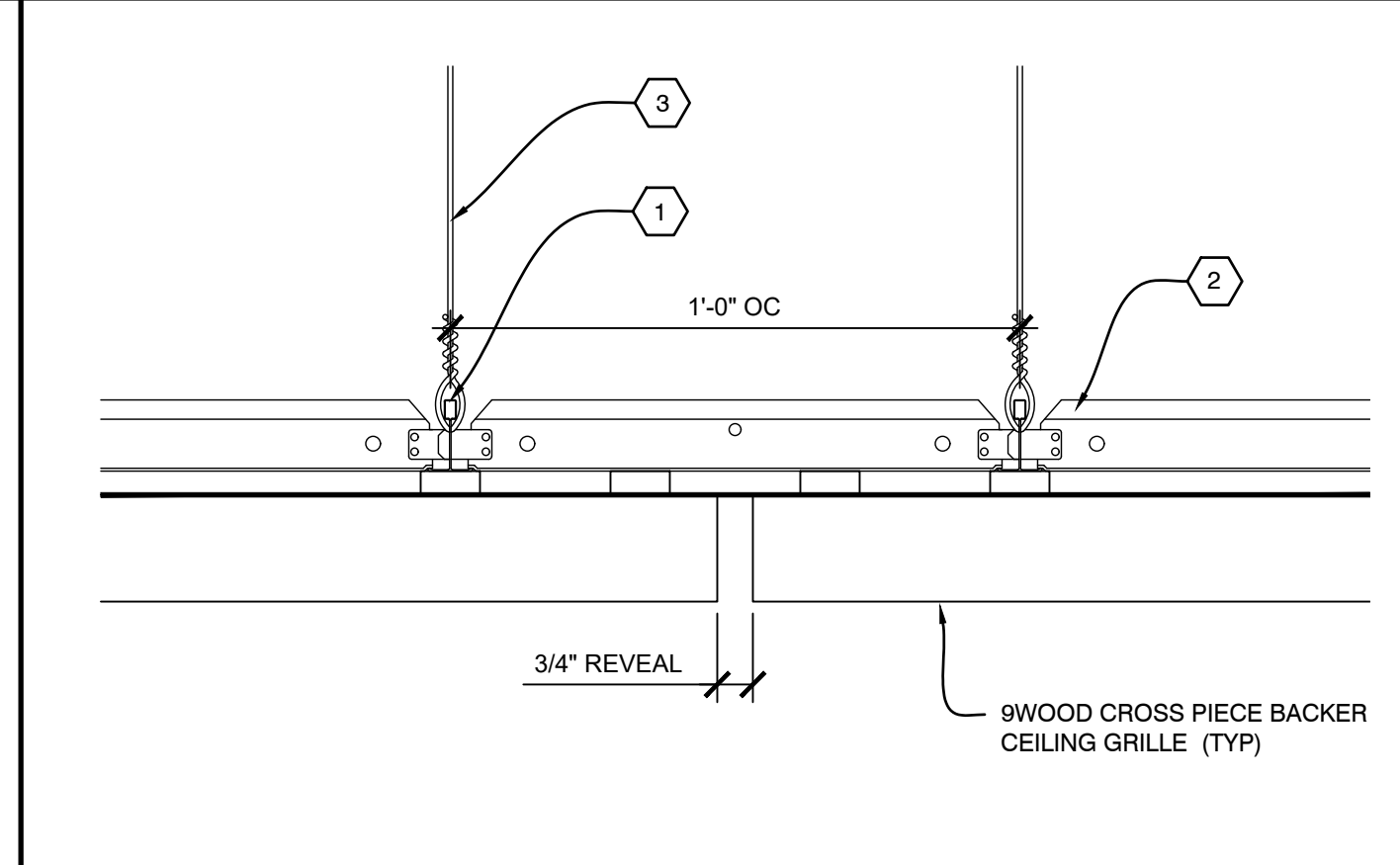
A3 SECTION - ABUTTING REVEAL SCALE: 1/4" = 1'
