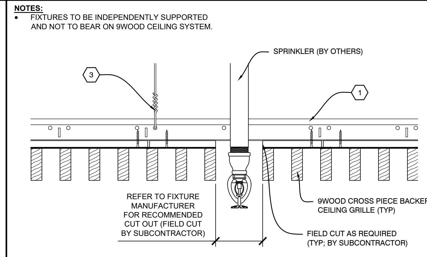
B3 SECTION - SPRINKLER SCALE: 1/4" = 1'
