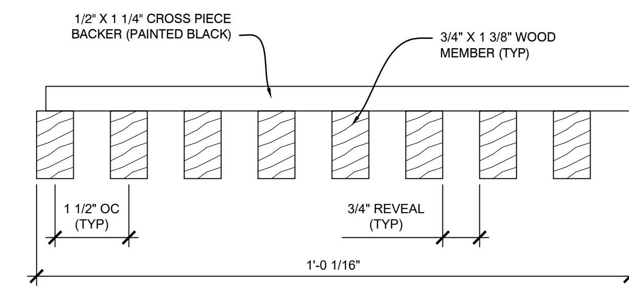
C3 SECTION - CROSS PIECE BACKER WOOD GRILLE SCALE: 1/2" = 1"
