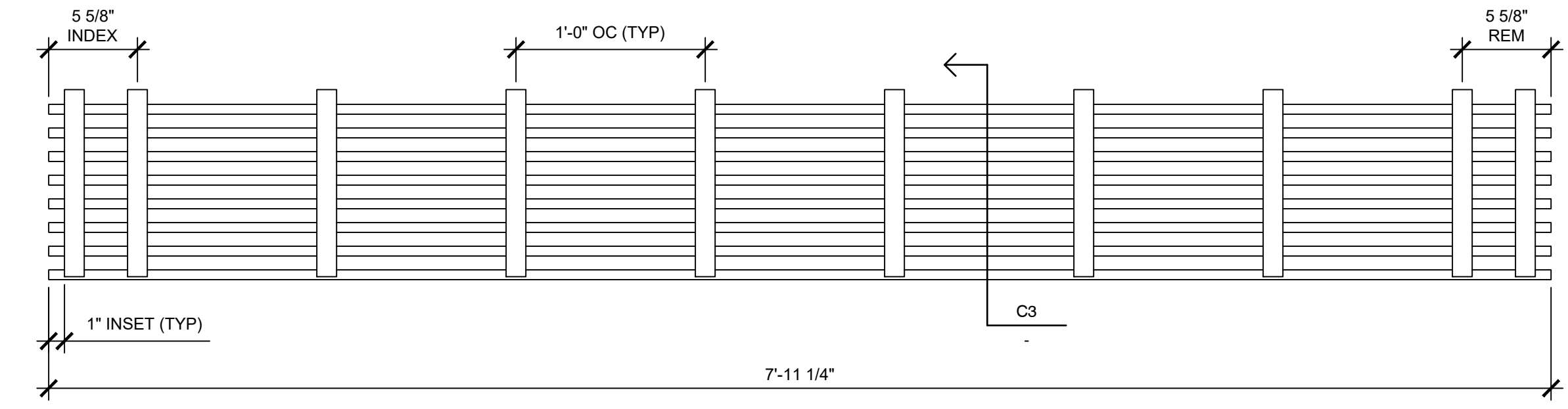
D3 PLAN VIEW - CROSS PIECE BACKER WOOD GRILLE SCALE: 1 1/2" = 1"
