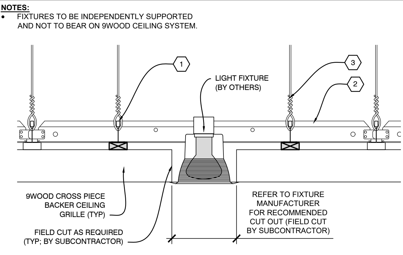
A2 SECTION - LIGHT FIXTURE SCALE: 1/4" = 1"
