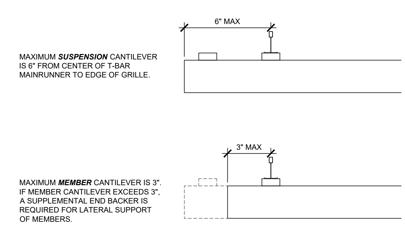
C4 SECTION - CANTILEVER RULES SCALE: 1/4" = 1"
