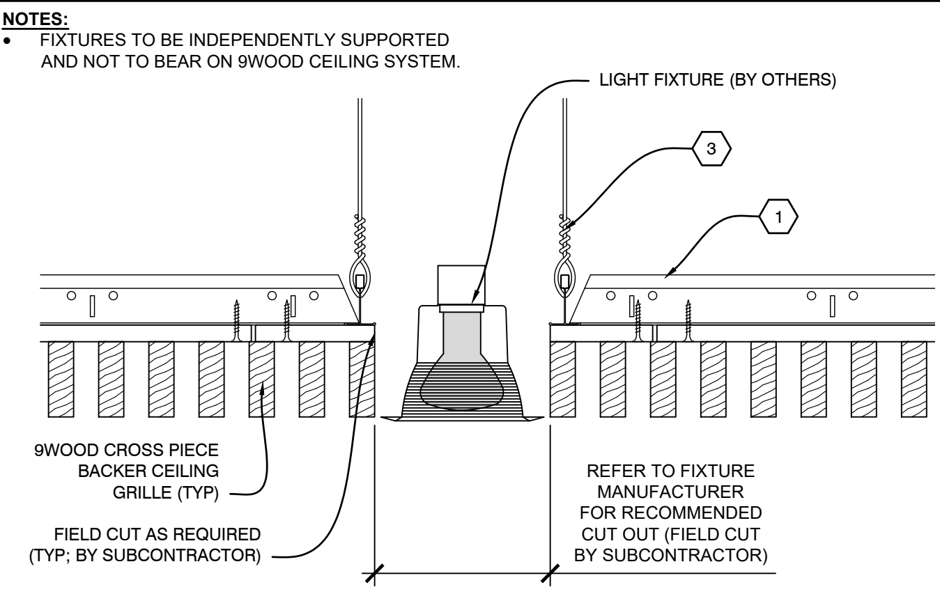
B2 SECTION - LIGHT FIXTURE SCALE: 1/4" = 1"
