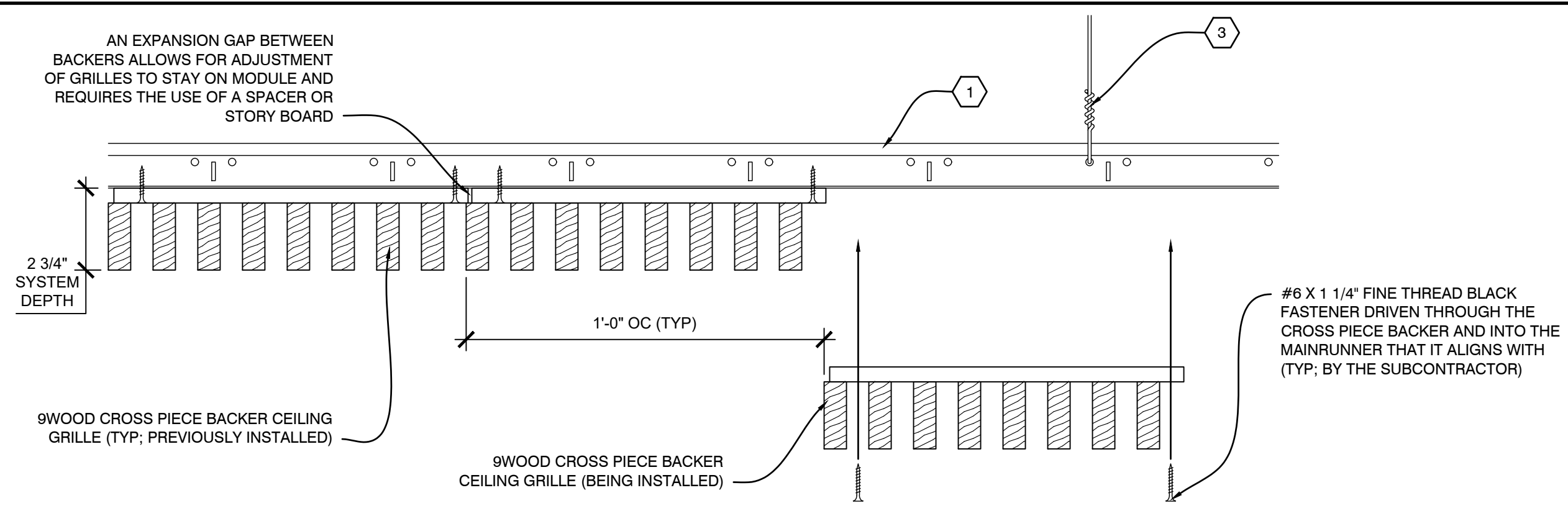
C1 INSTALLATION PROCESS - CROSS PIECE BACKER WOOD GRILLE SCALE: 1/4" = 1"
