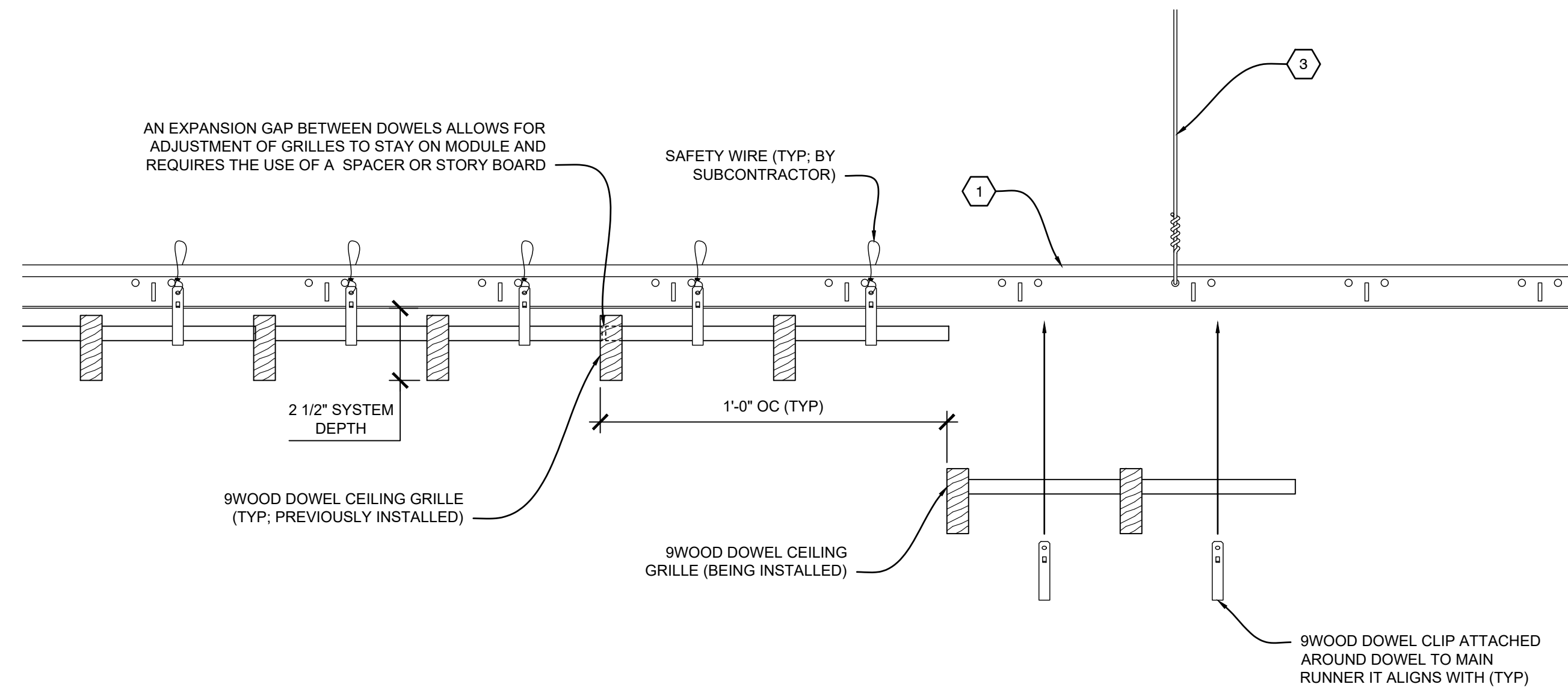
C3 INSTALLATION PROCESS - DOWEL CEILING GRILLE SCALE: 1/4" = 1'
