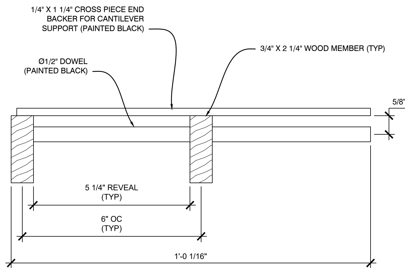
B1 SECTION - DOWEL CEILING GRILLE SCALE: 1/2" = 1'
