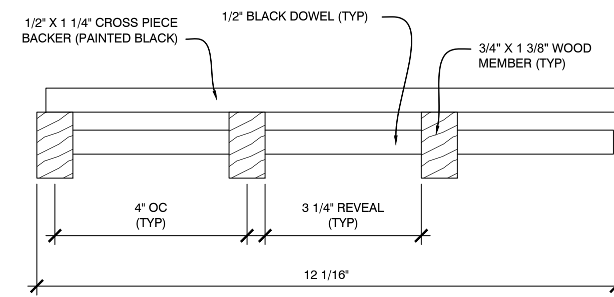
C3 SECTION - CROSS PIECE BACKER WOOD GRILLE SCALE: 1/2" = 1"
