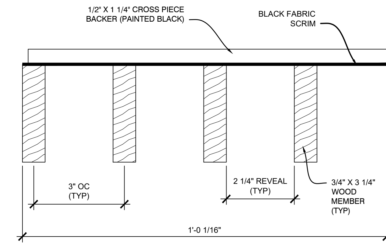
C3 SECTION - CROSS PIECE BACKER WOOD GRILLE SCALE: 1/2" = 1"
