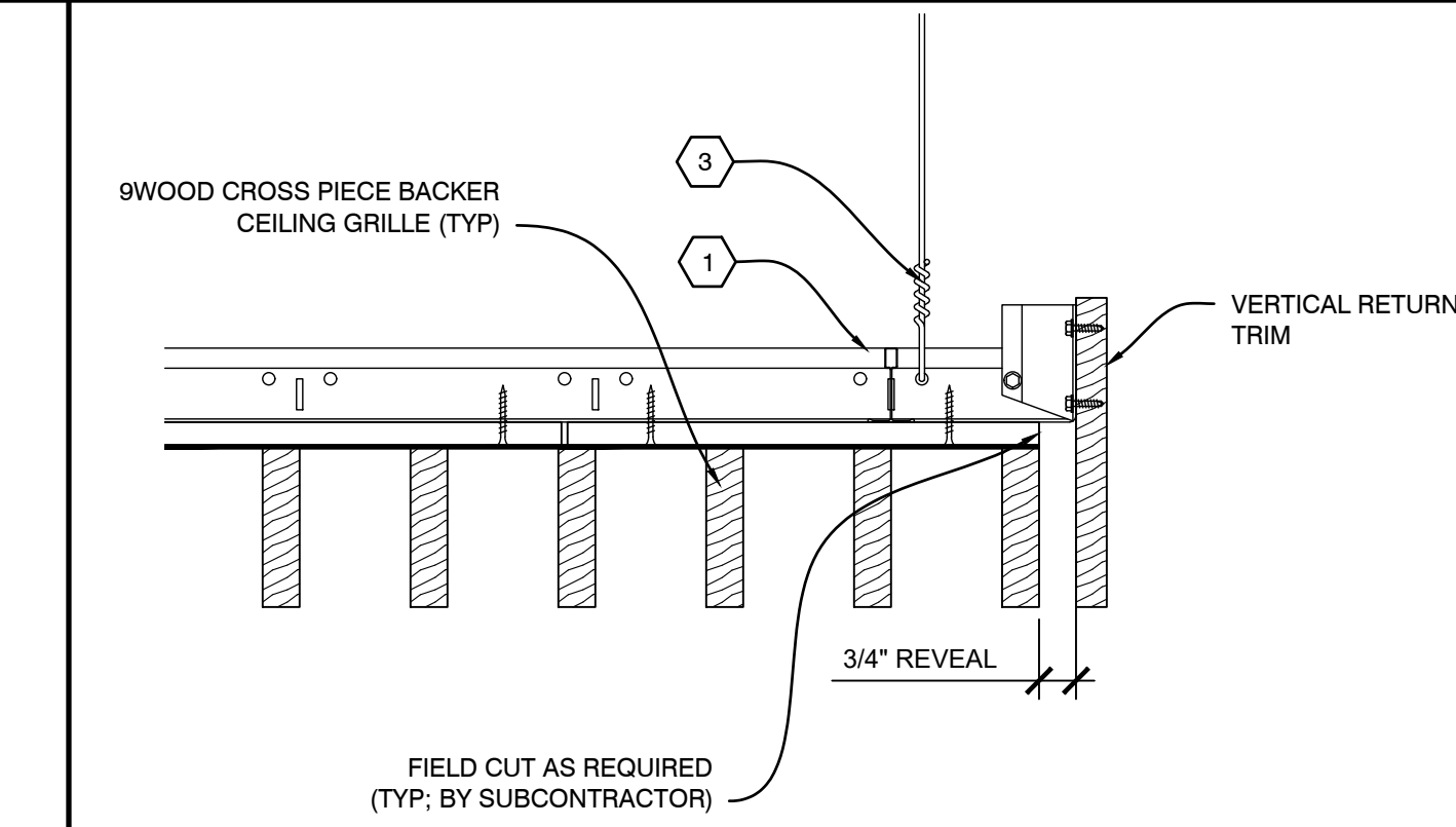
B4 SECTION - PERIMETER SCALE: 1/4" = 1"
