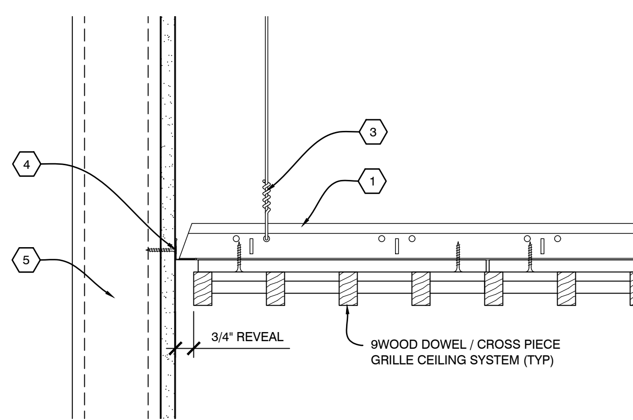
B1 SECTION - PERIMETER SCALE: 1/4" = 1"
