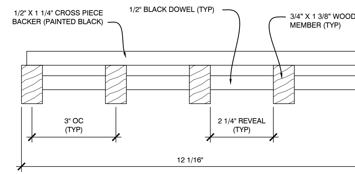
C3 SECTION - CROSS PIECE BACKER WOOD GRILLE SCALE: 1/2" = 1"
