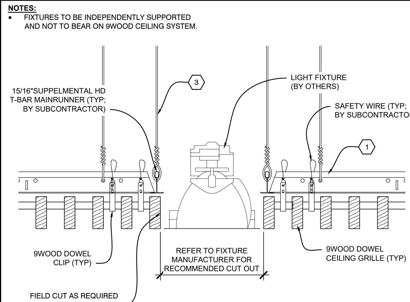
C3 INSTALLATION PROCESS - DOWEL CEILING GRILLE SCALE: 1/4" = 1'
