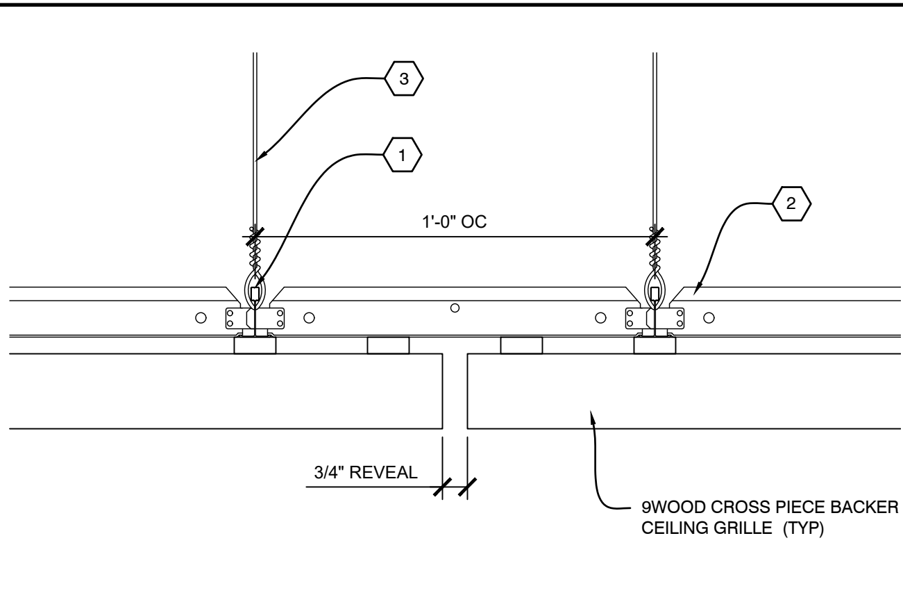
A3 SECTION - ABUTTING REVEAL SCALE: 1/4" = 1"
