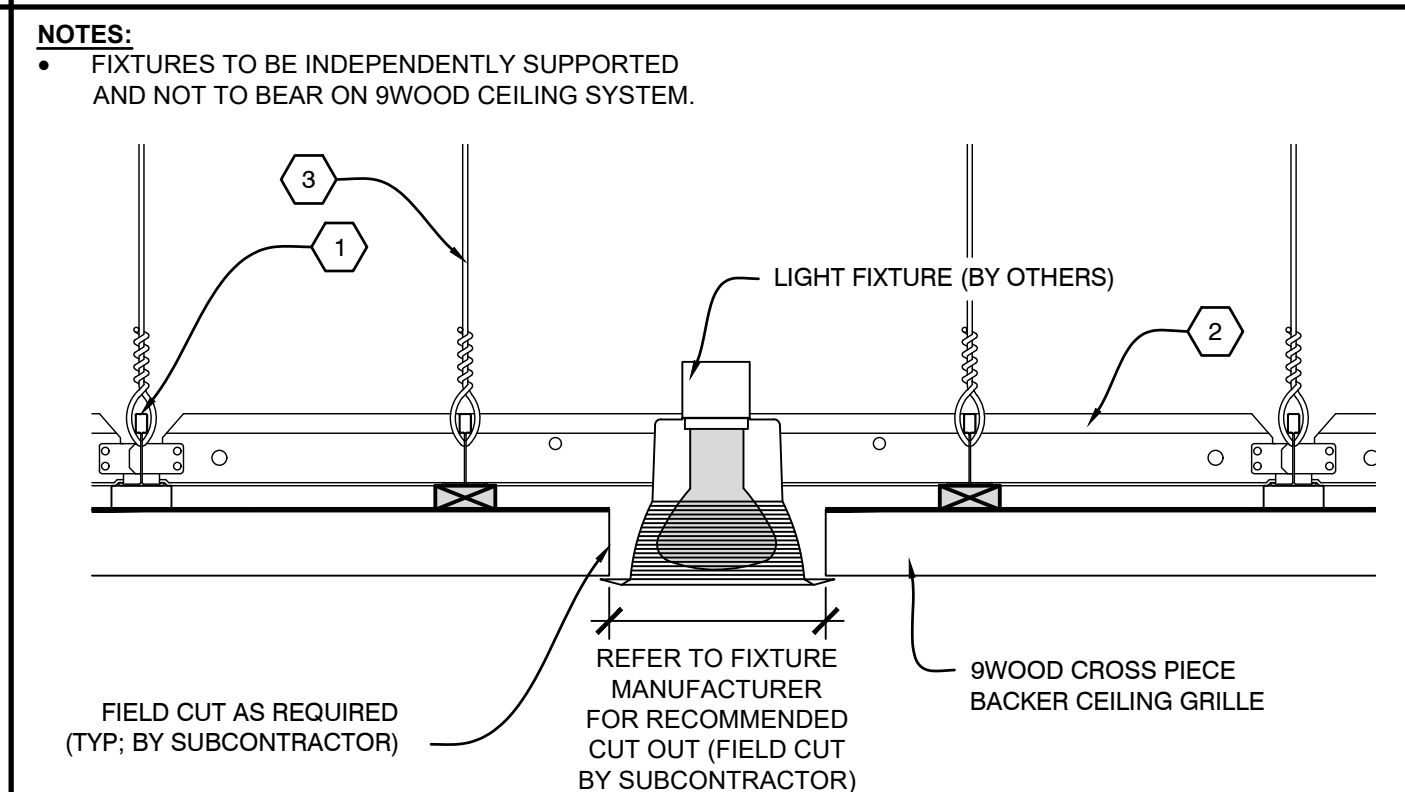
A2 SECTION - LIGHT FIXTURE SCALE: 1/4" = 1'
