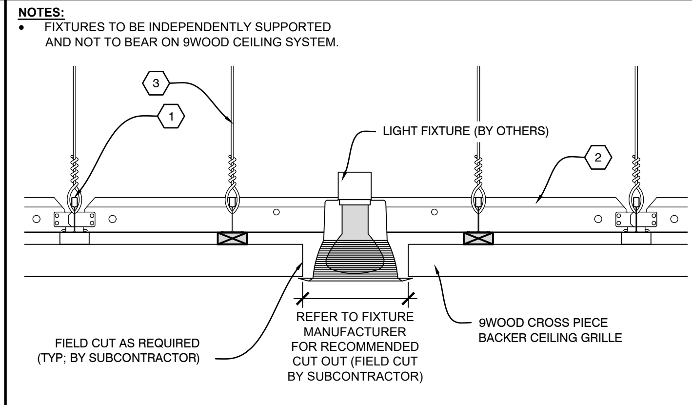
A2 SECTION - LIGHT FIXTURE SCALE: 1/4" = 1'
