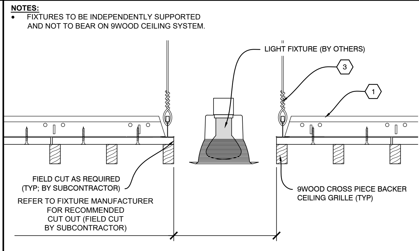
B2 SECTION - LIGHT FIXTURE SCALE: 1/4" = 1'
