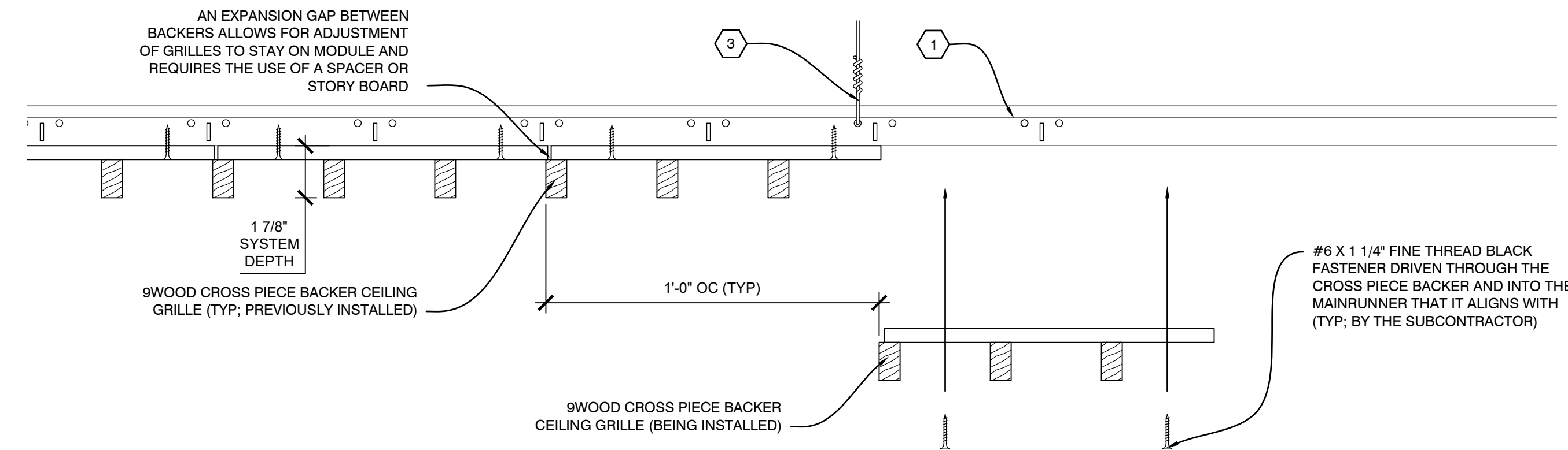
C1 INSTALLATION PROCESS - CROSS PIECE BACKER WOOD GRILLE SCALE: 1/4" = 1'
