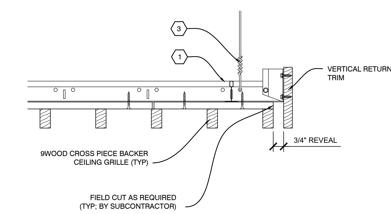
B4 SECTION - PERIMETER SCALE: 1/4" = 1'
