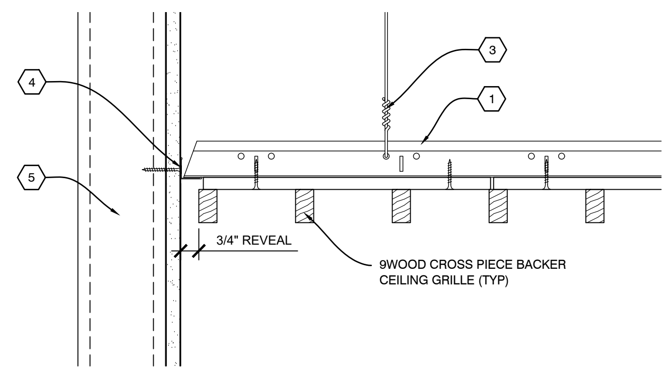
B1 SECTION - PERIMETER SCALE: 1/4" = 1'
