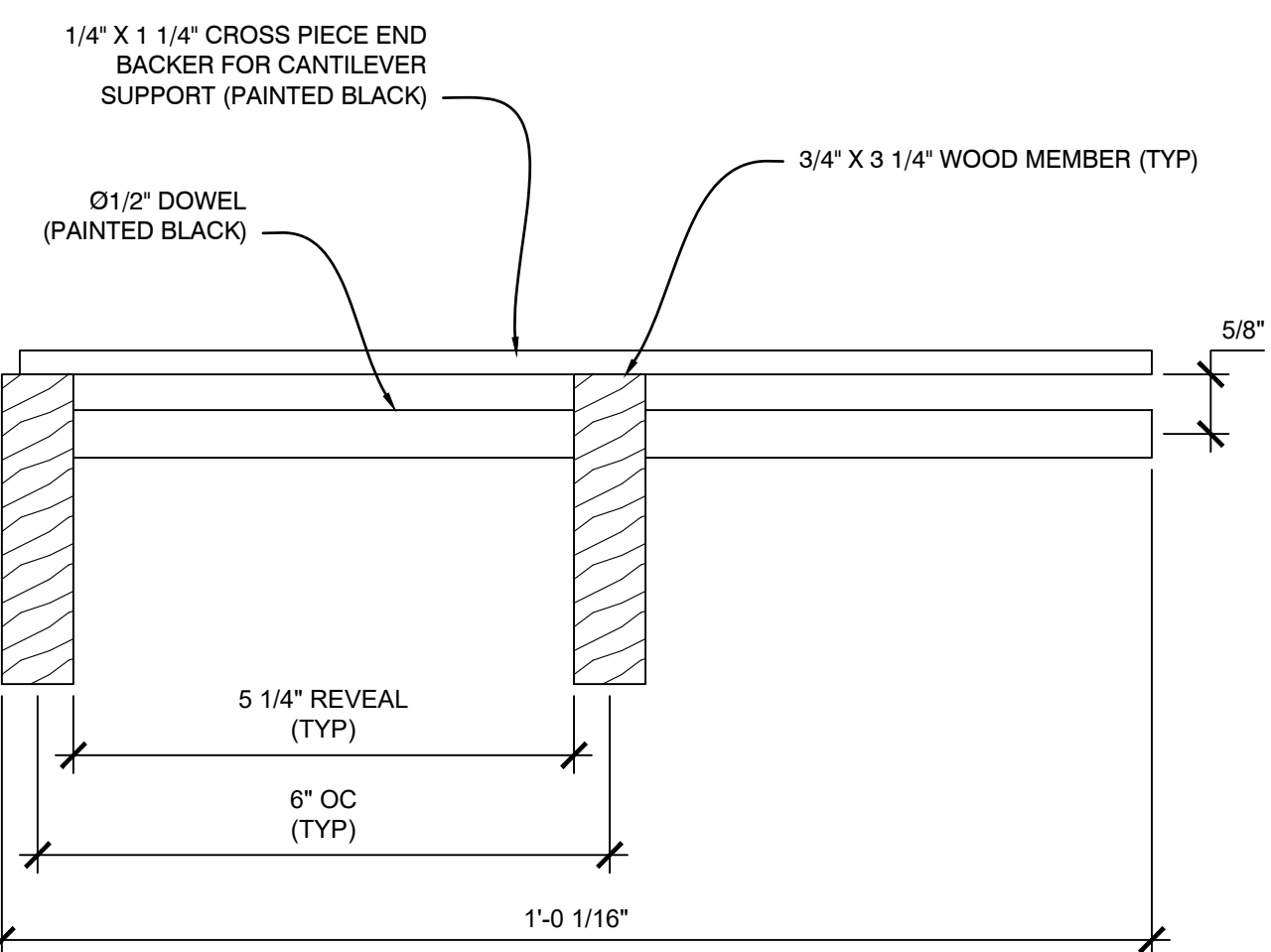
B1 SECTION - DOWEL CEILING GRILLE SCALE: 1/2" = 1"
