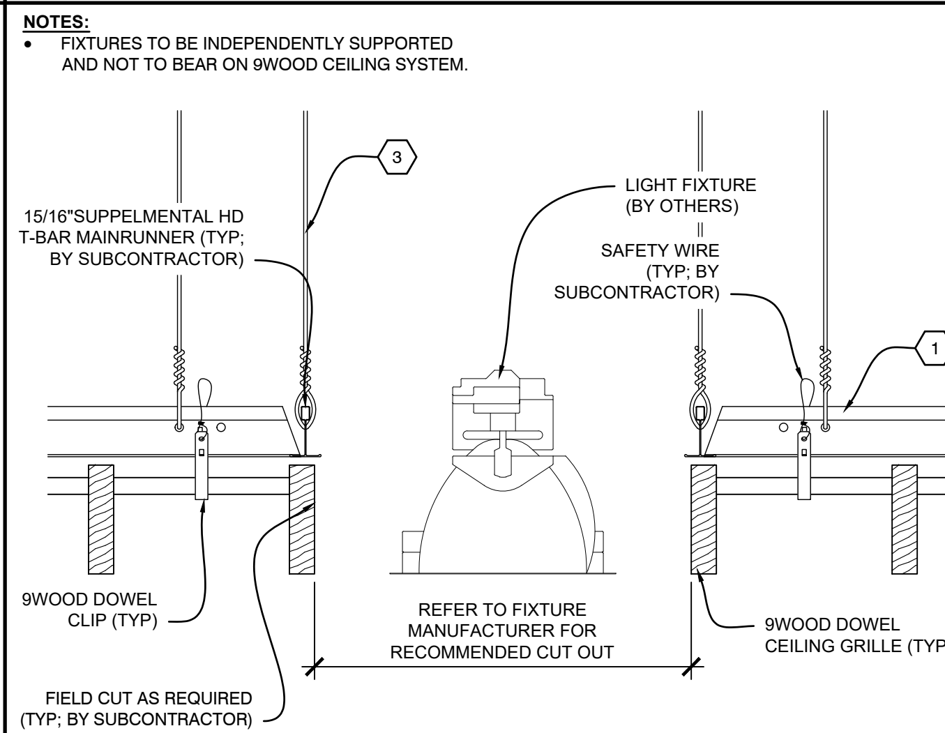
C3 INSTALLATION PROCESS - DOWEL CEILING GRILLE SCALE: 1/4" = 1"
