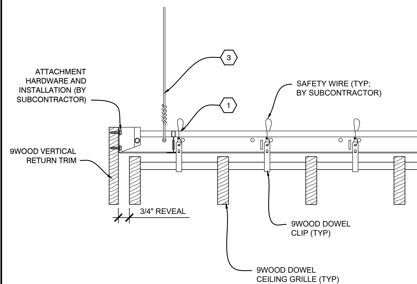
B2 SECTION - PERIMETER SCALE: 1/4" = 1"
