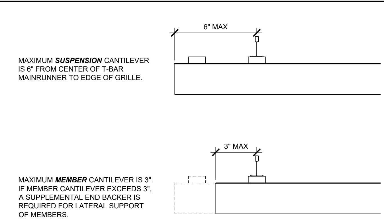
C4 SECTION - CANTILEVER RULES SCALE: 1/4" = 1'
