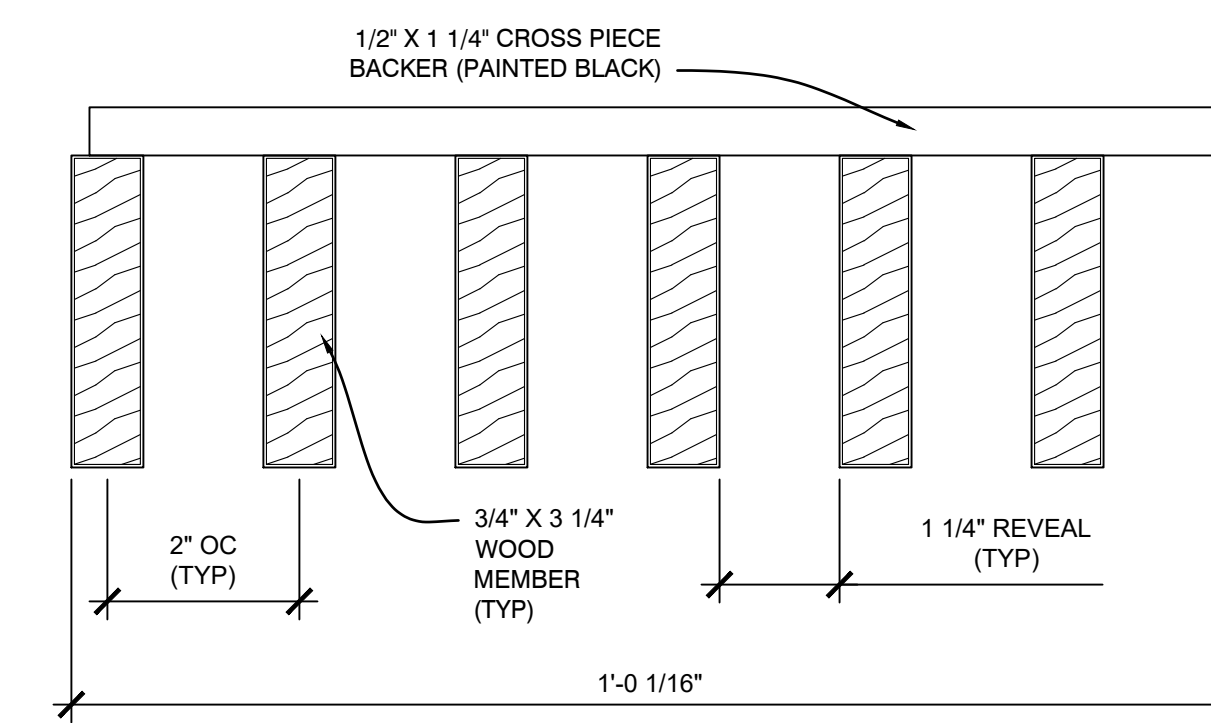
C3 SECTION - CROSS PIECE BACKER WOOD GRILLE SCALE: 1/2" = 1'
