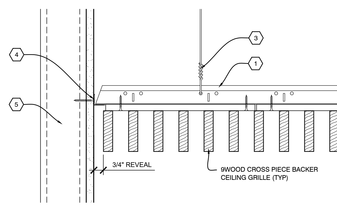
B1 SECTION - PERIMETER SCALE: 1/4" = 1'
