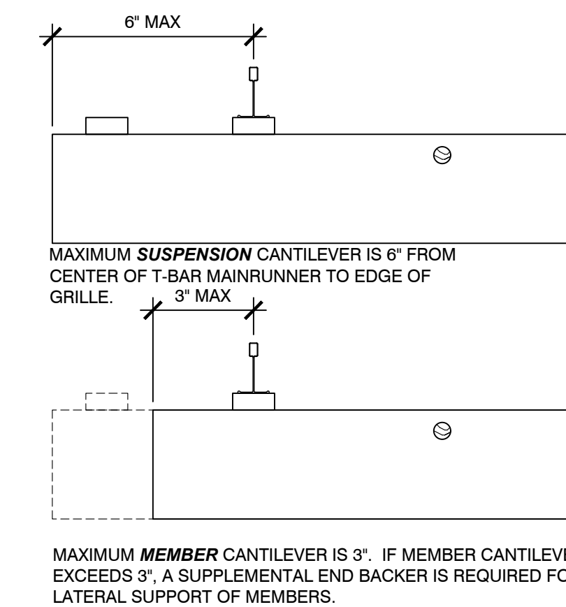
C4 SECTION - CANTILEVER RULES SCALE: 1/4" = 1"
