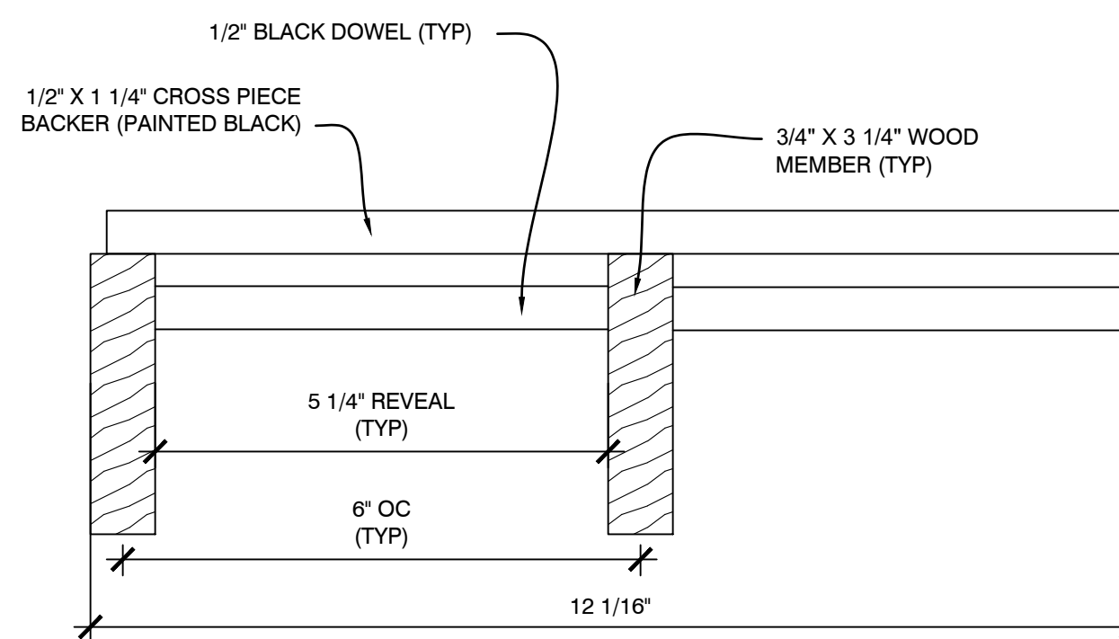
C3 SECTION - CROSS PIECE BACKER WOOD GRILLE SCALE: 1/2" = 1"
