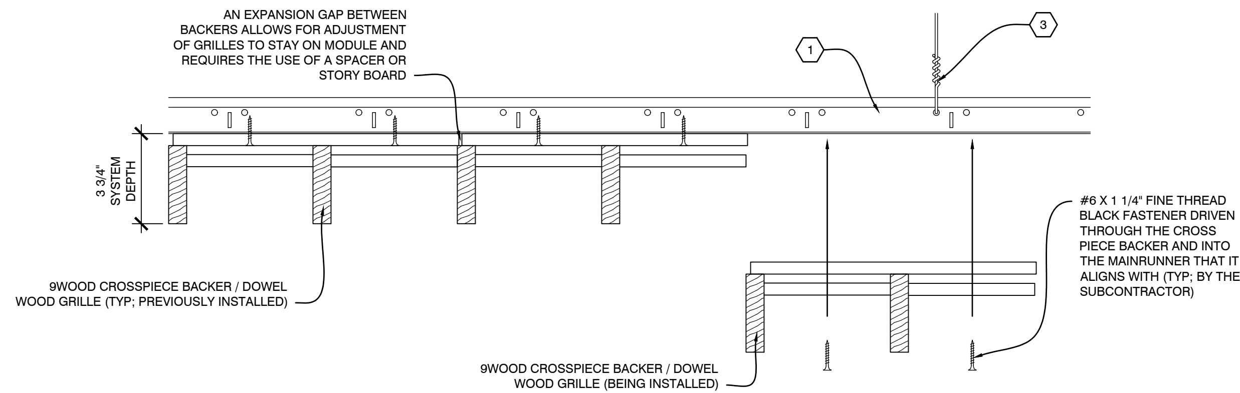
C1 INSTALLATION PROCESS - CROSS PIECE BACKER WOOD GRILLE SCALE: 1/4" = 1"
