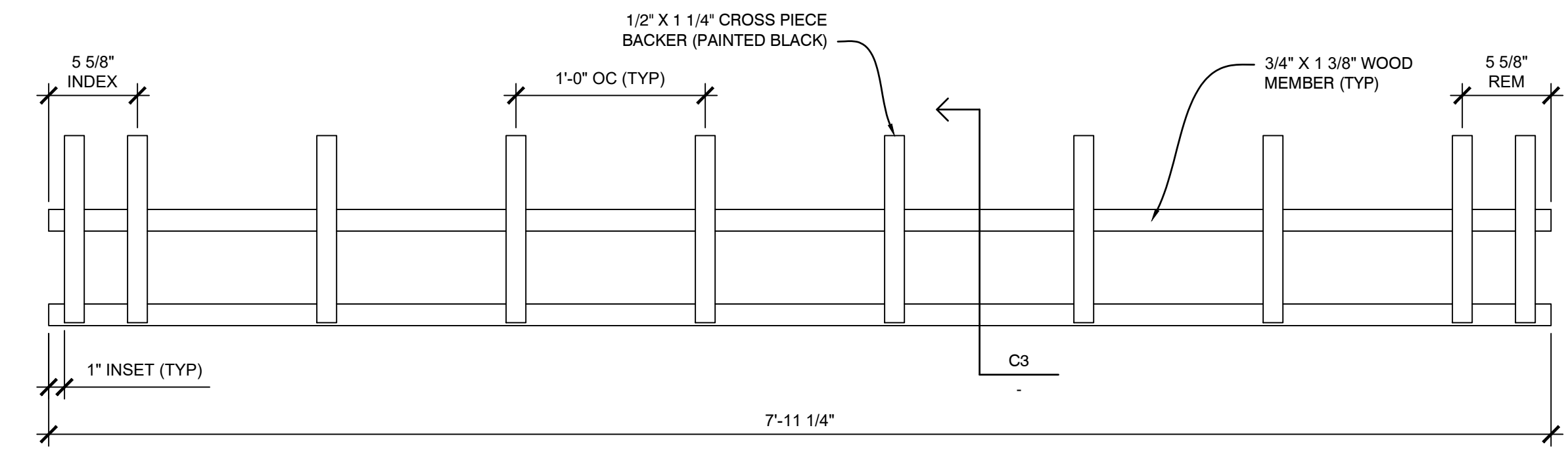
D3 PLAN VIEW - LINEAR CEILING PANEL SCALE: 1 1/2" = 1'
