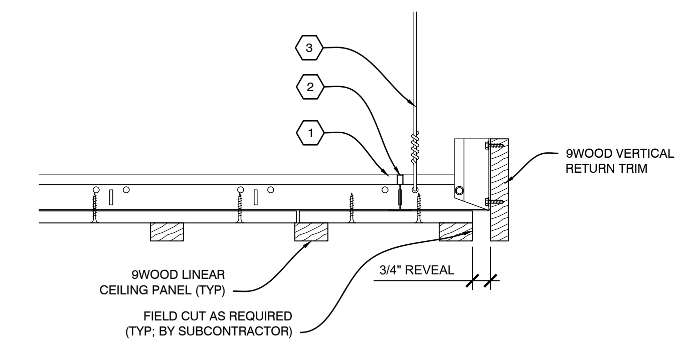
B4 SECTION - PERIMETER SCALE: 1/4" = 1'
