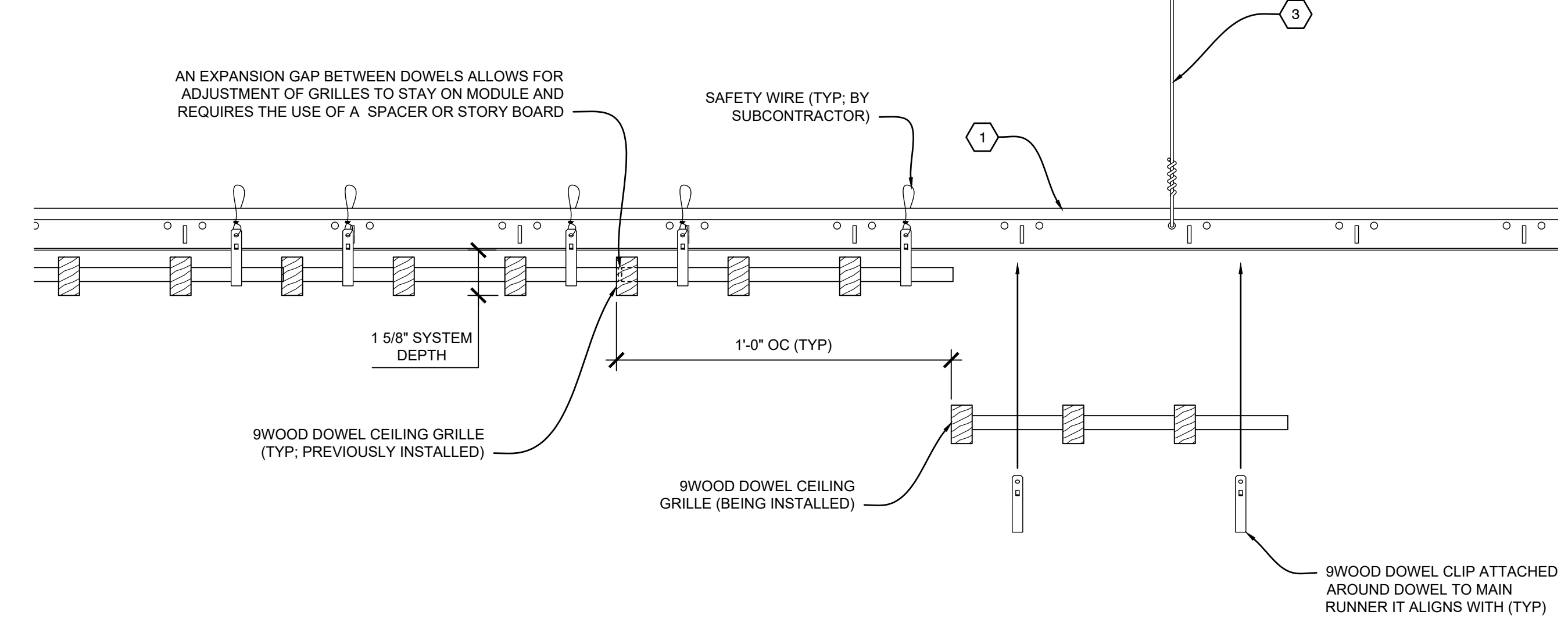
C3 INSTALLATION PROCESS - DOWEL CEILING GRILLE SCALE: 1/4" = 1'
