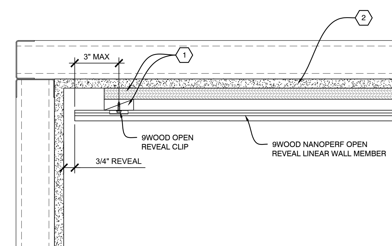
A1 PLAN VIEW - PERIMETER SCALE: 1/4" = 1' 0 2' 4' 8'
