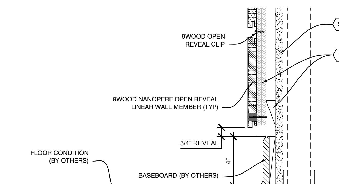
B4 SECTION - FLOOR PERIMETER
