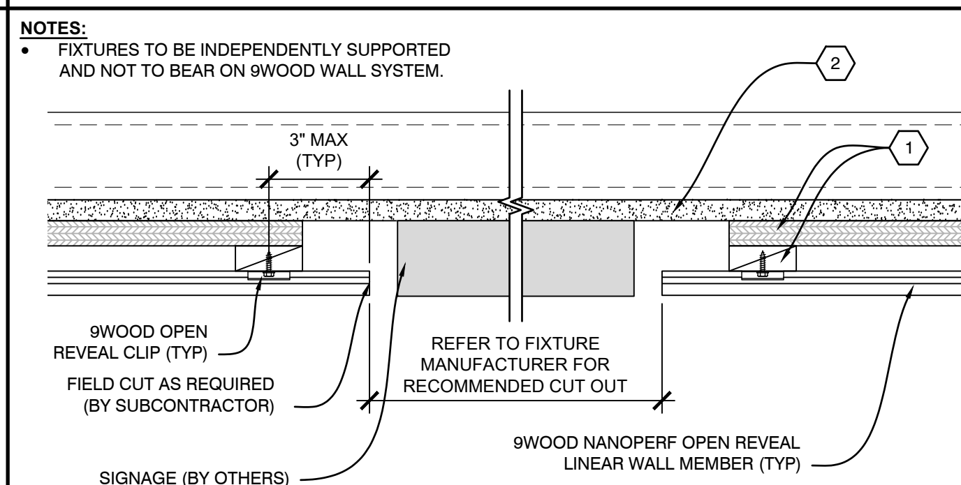
FACE / PLAN VIEW - NANOPERF OPEN REVEAL LINEAR MEMBER
