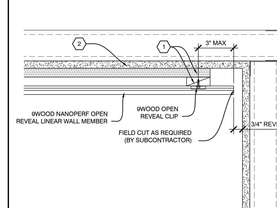
A4 PLAN VIEW - PERIMETER SCALE: 1/4" = 1' 0 2' 4'
