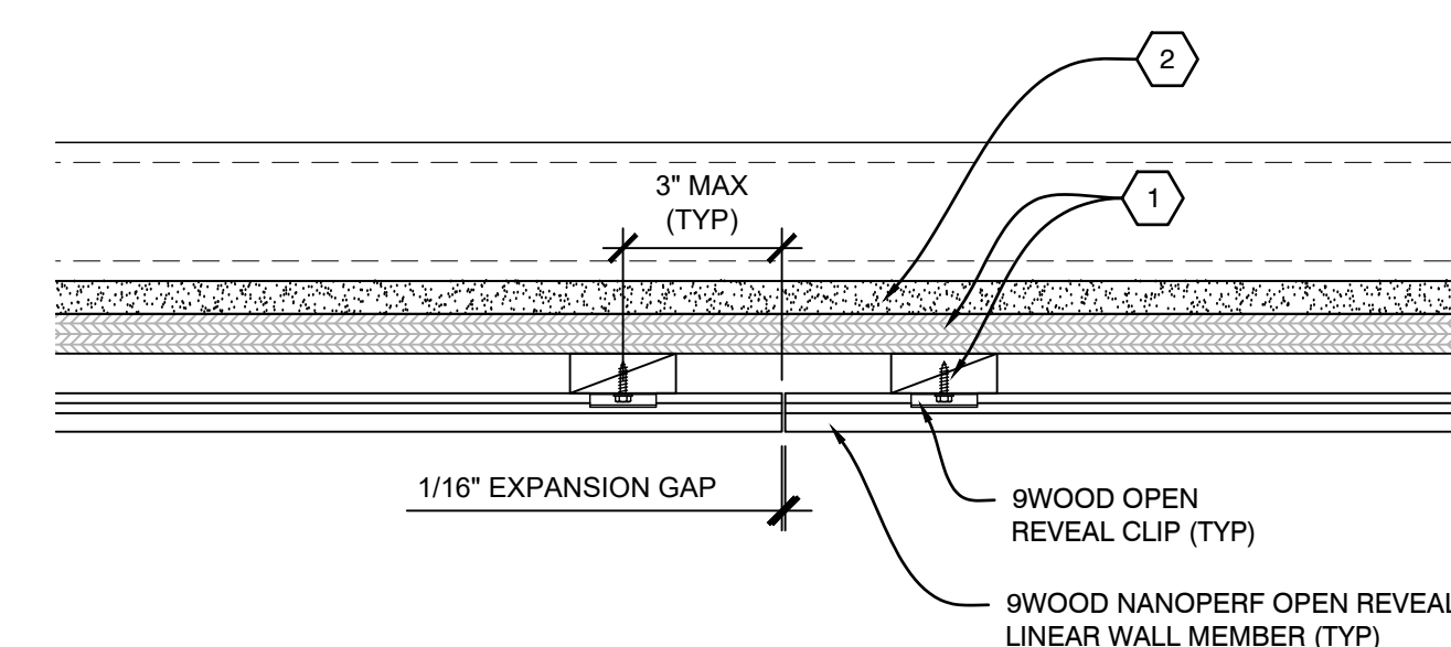
INSTALLATION PROCESS - NANOPERF OPEN REVEAL LINEAR MEMBER
