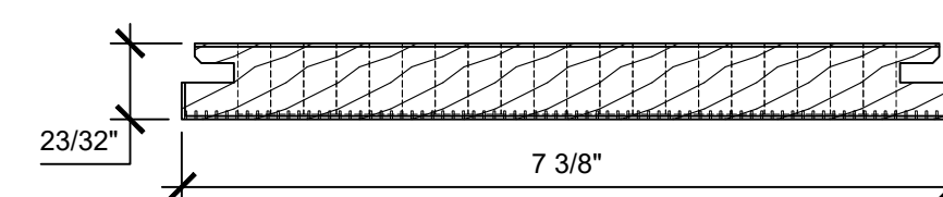
SECTION - NANOPERF OPEN REVEAL LINEAR MEMBER
