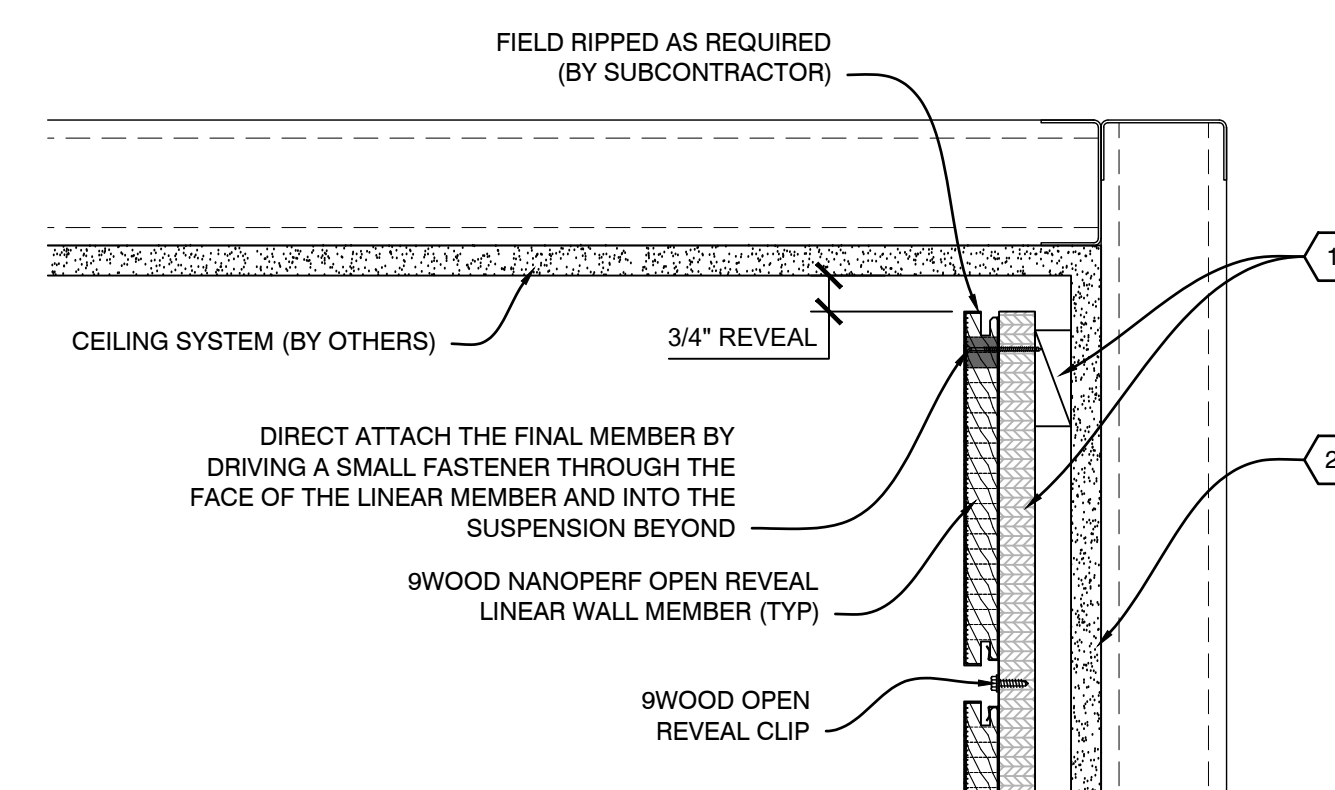
SECTION - CEILING PERIMETER
