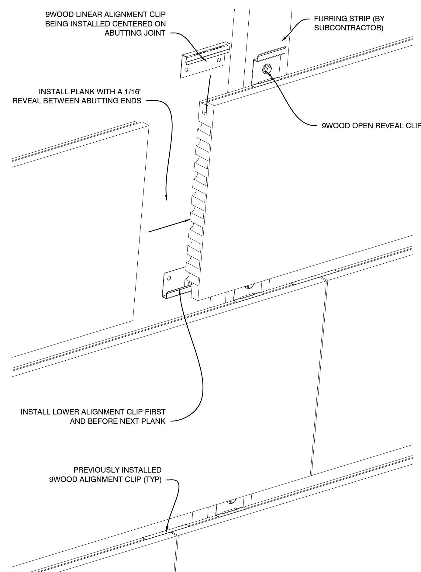
B1 ISO VIEW - INSTALLATION SCALE: NOT TO SCALE
