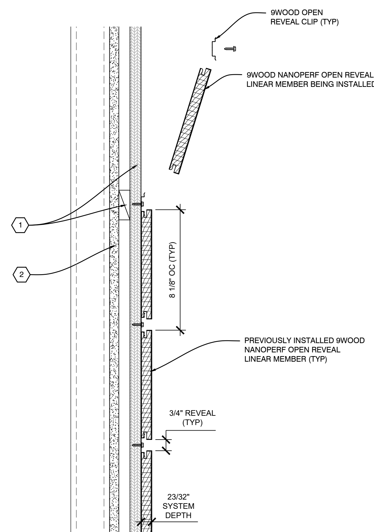
INSTALLATION PROCESS - NANOPERF OPEN REVEAL LINEAR MEMBER
